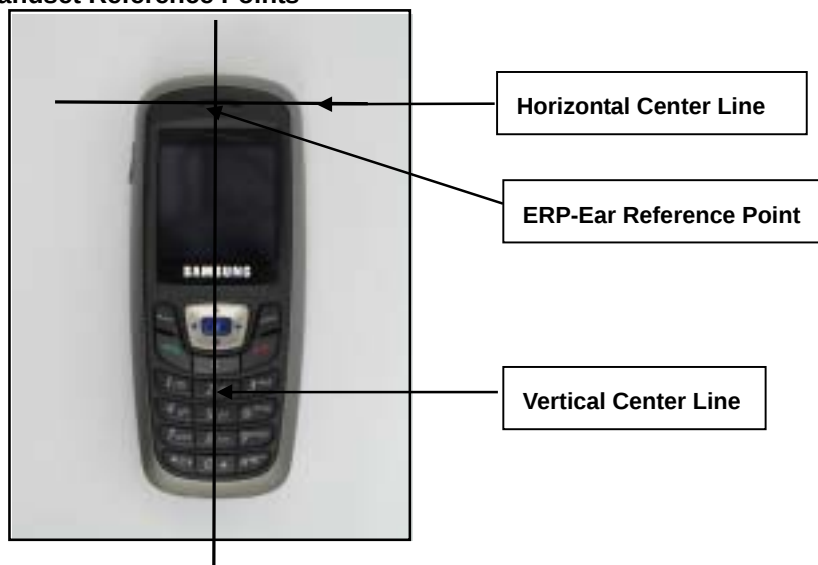
Figure 8.1 Handset Reference Points
