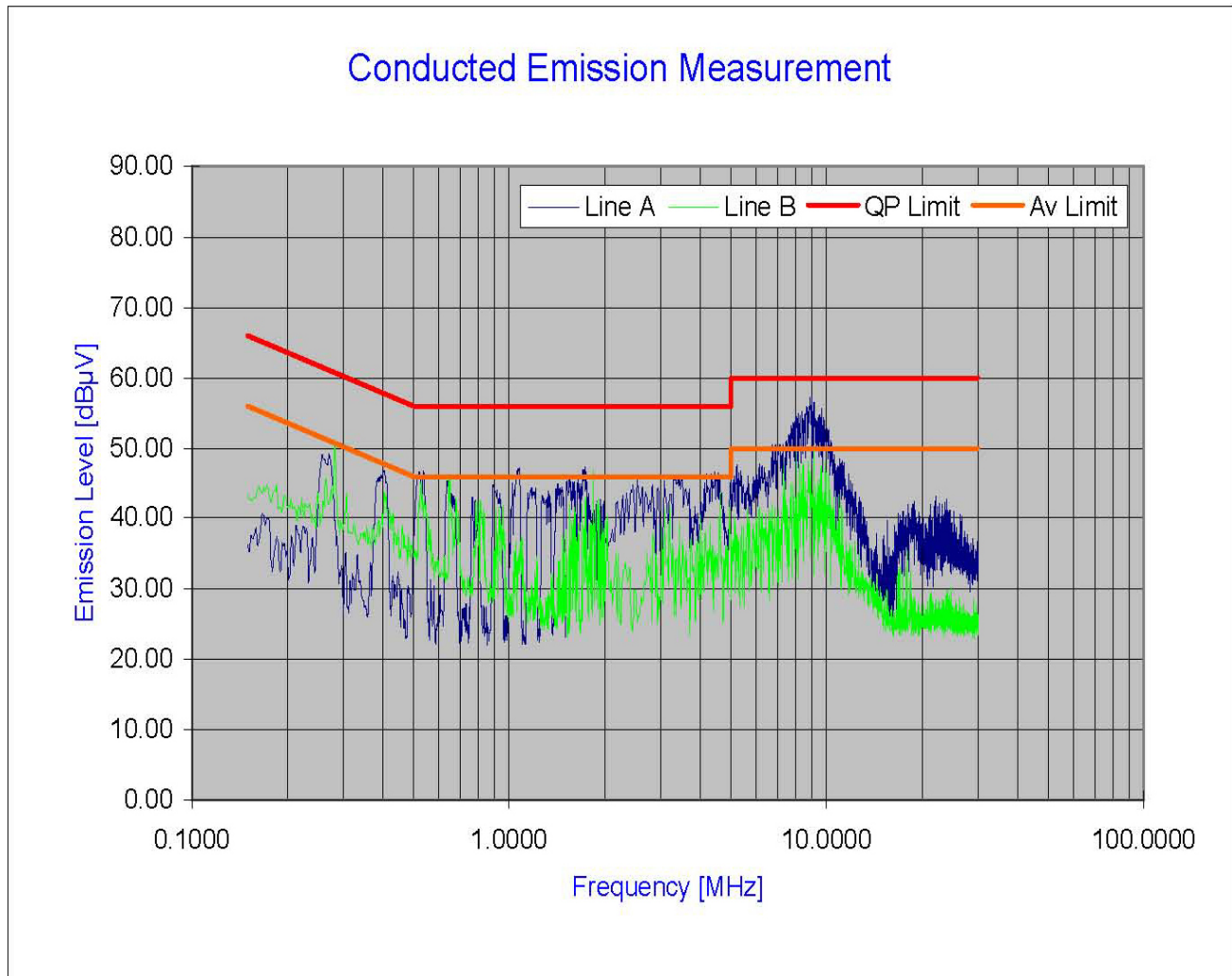
Plot 7-1. Line-Conducted Test Plot
