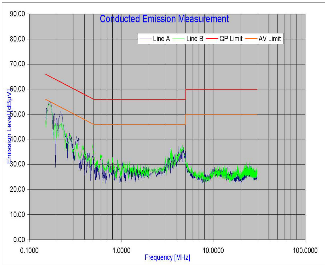
Plot 7-1. Line-Conducted Test Plot
