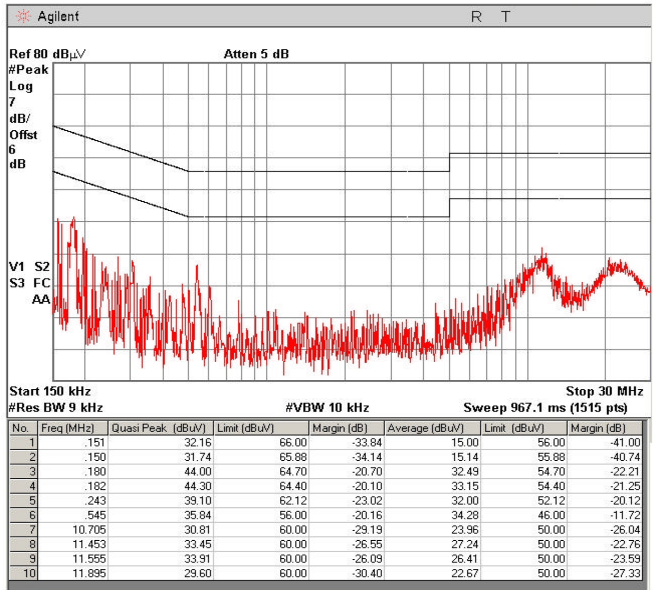
Plot 7-4. Line-Conducted Test Plot – Line B
