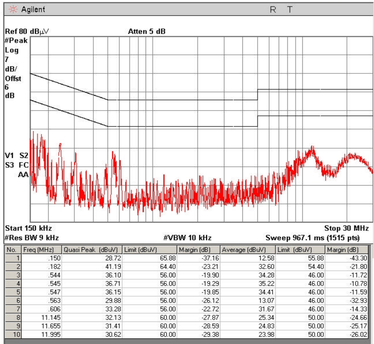
Plot 7-3. Line-Conducted Test Plot – Line A
