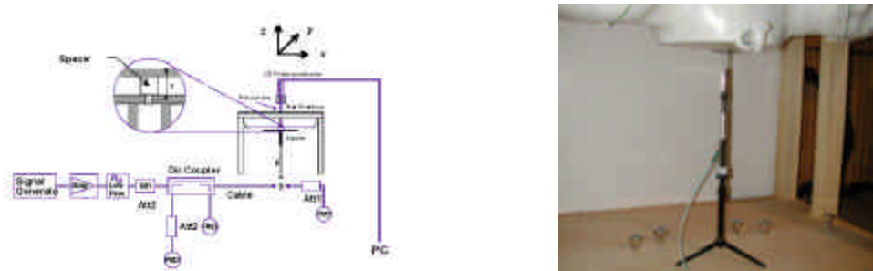
Figure 12.1 Dipole Validation Test Setup
