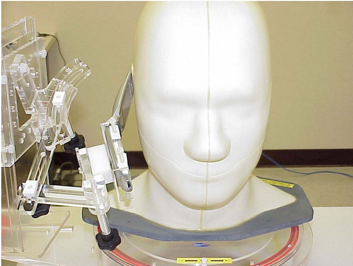
Photo 7. Right tilt
