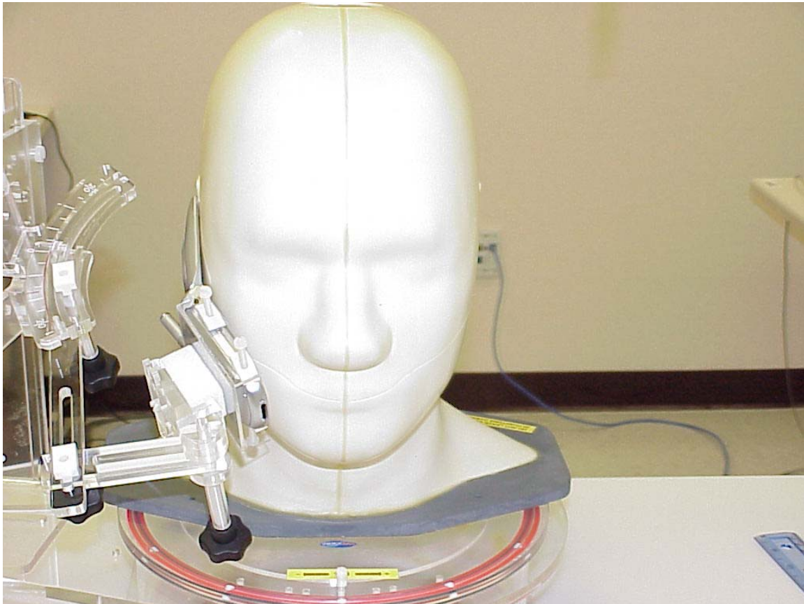
Photo 6. Right touch
