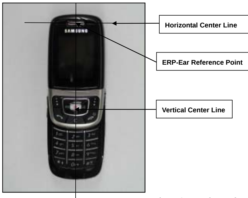
Figure 8.1 Handset Reference Points
