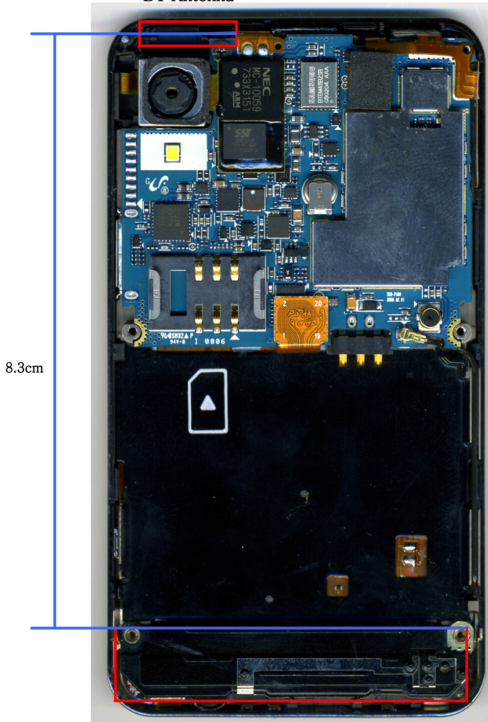
Main Antenna
