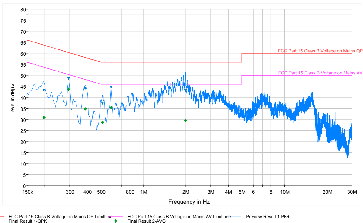
Plot 6-63. Line Conducted Plot with 802.11b (L1)
