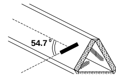
Figure 3.3 Triangular Probe Configuration
