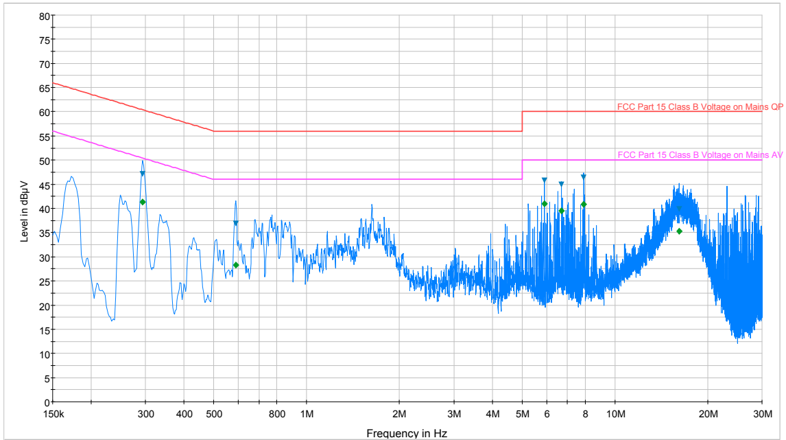
Plot 6-69. Line Conducted Plot with 802.11a (L1)
