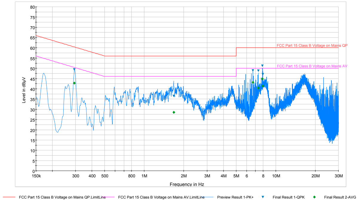
Plot 6-68. Line Conducted Plot with 802.11b (N)
