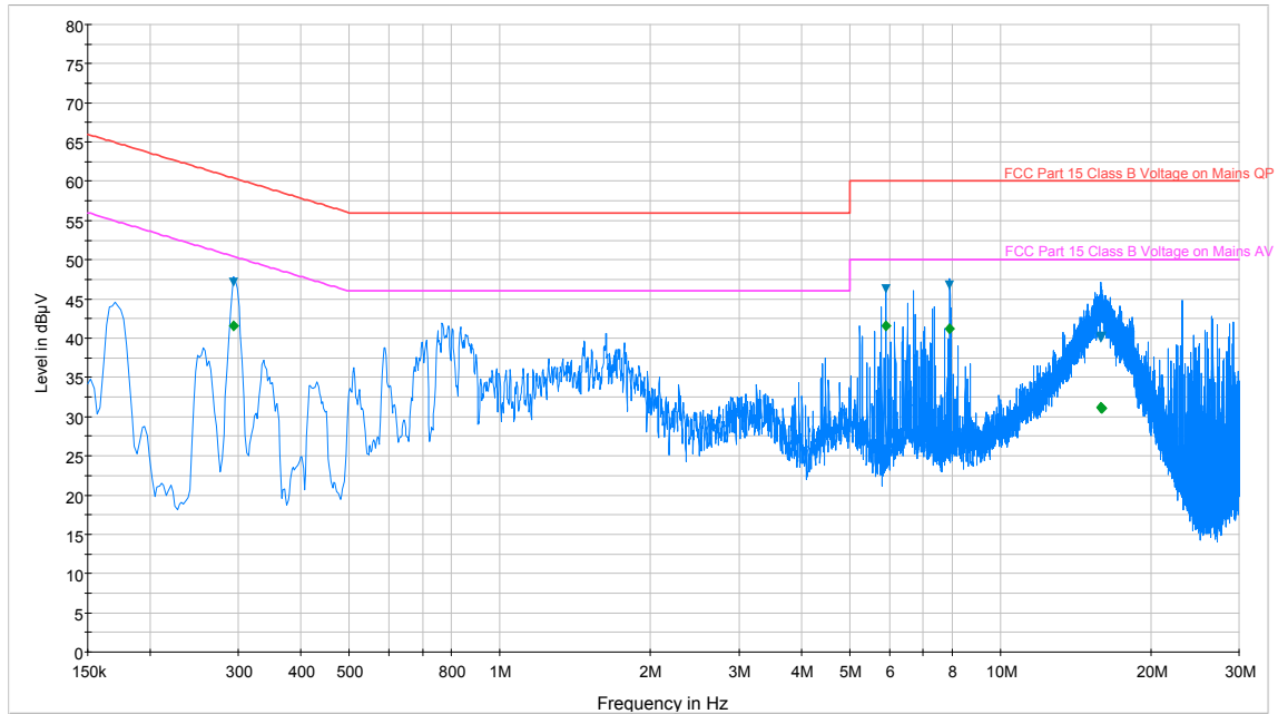
Plot 6-70. Line Conducted Plot with 802.11a (N)
