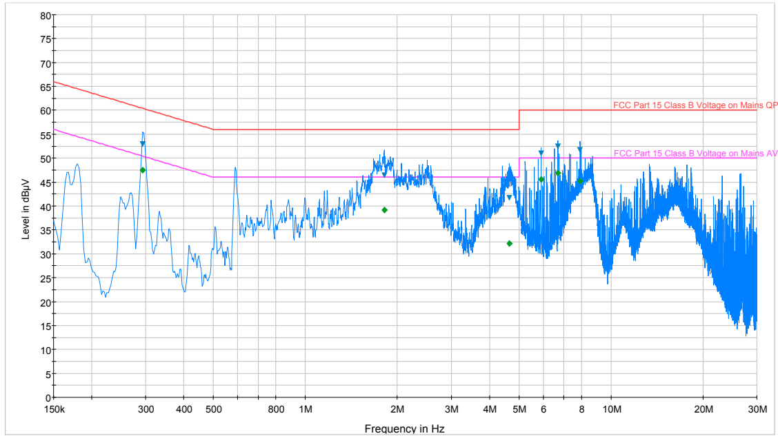
Plot 6-67. Line Conducted Plot with 802.11b (L1)
