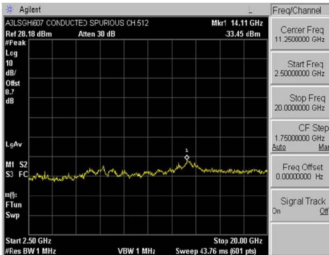
Plot A-12. Conducted Spurious Plot (PCS GSM Mode – Ch. 512)
