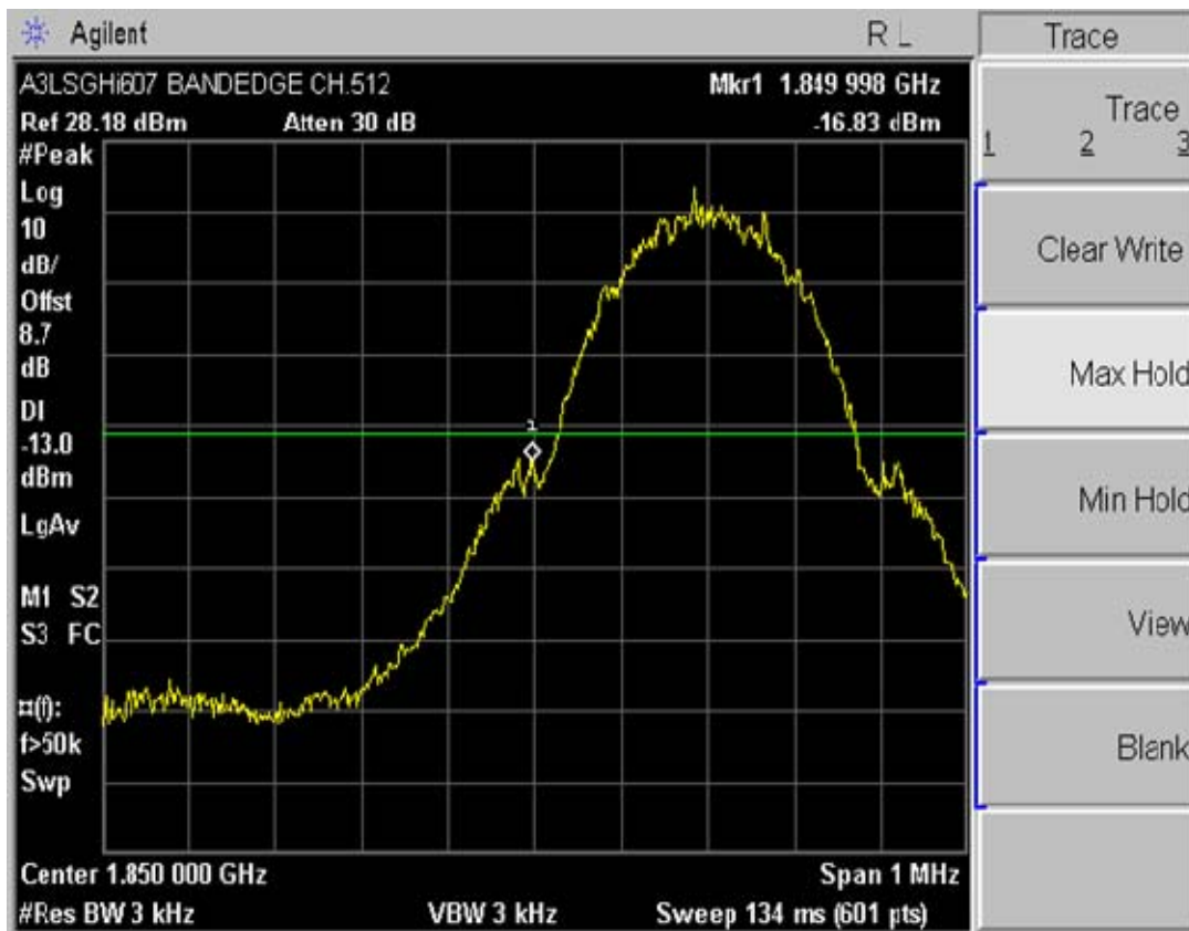
Plot A-13. Band Edge Plot (PCS GSM Mode – Ch. 512)
