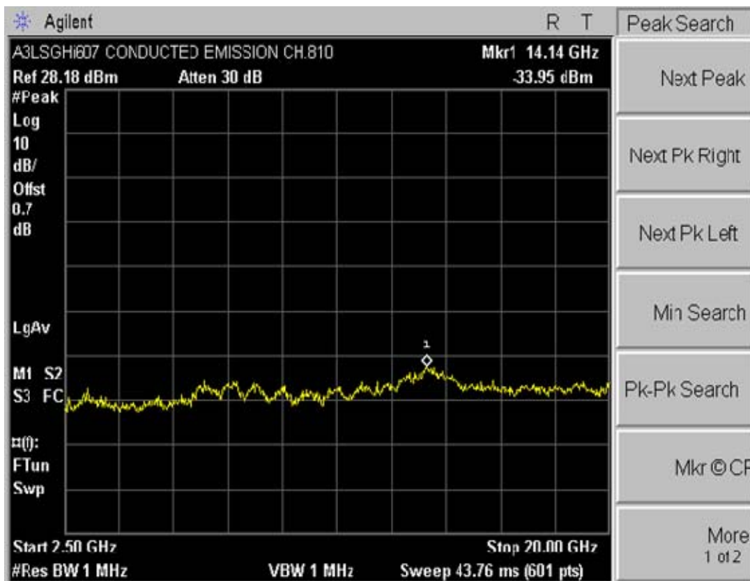
Plot A-18. Conducted Spurious Plot (PCS GSM Mode – Ch. 810)
