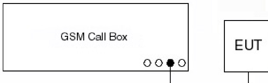
Figure 6-1. GSM Conducted Power Test Setup Diagram
