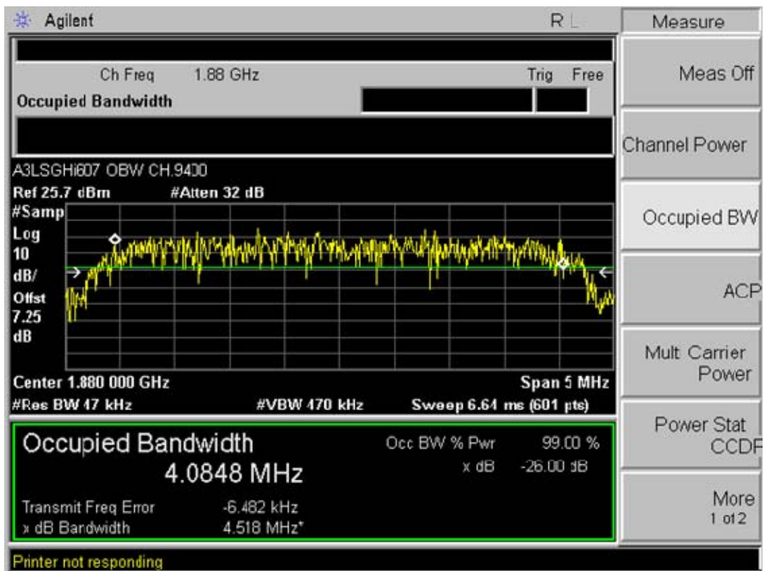
Plot A-19. Occupied Bandwidth Plot (PCS WCDMA Mode – Ch. 9400)
