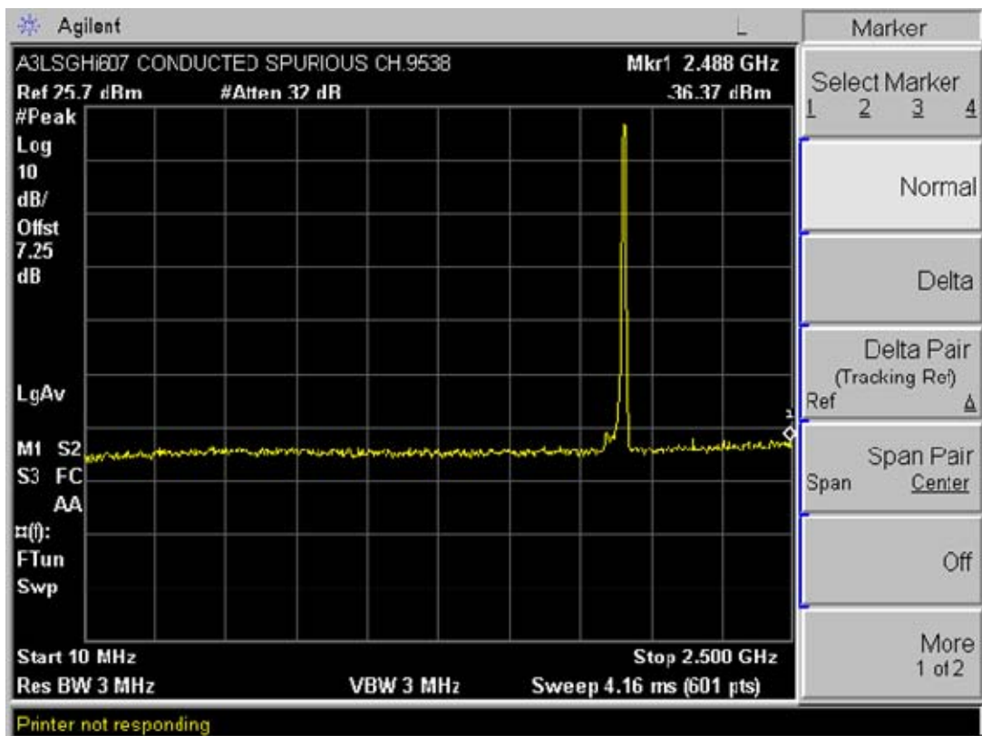
Plot A-21. Conducted Spurious Plot (PCS WCDMA Mode – Ch. 9538)
