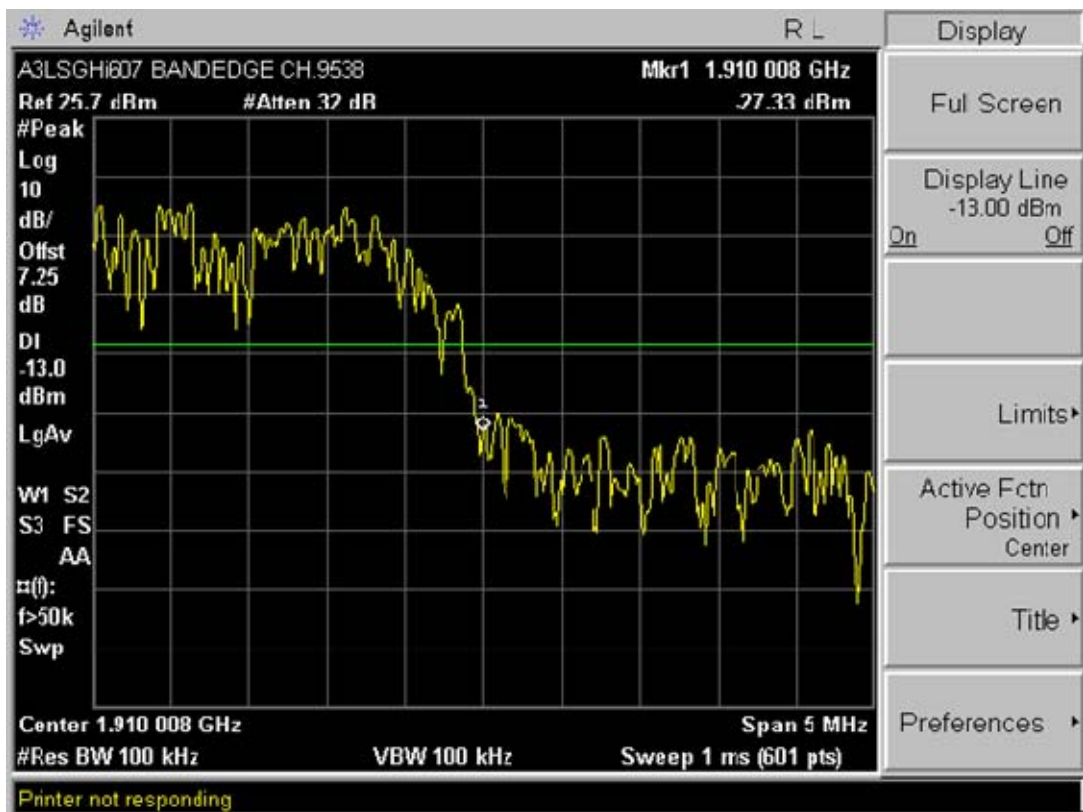
Plot A-23. Band Edge Plot (PCS WCDMA Mode – Ch. 9538)
