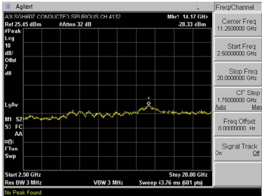
Plot A-2. Conducted Spurious Plot (Cellular WCDMA Mode – Ch. 4132)
