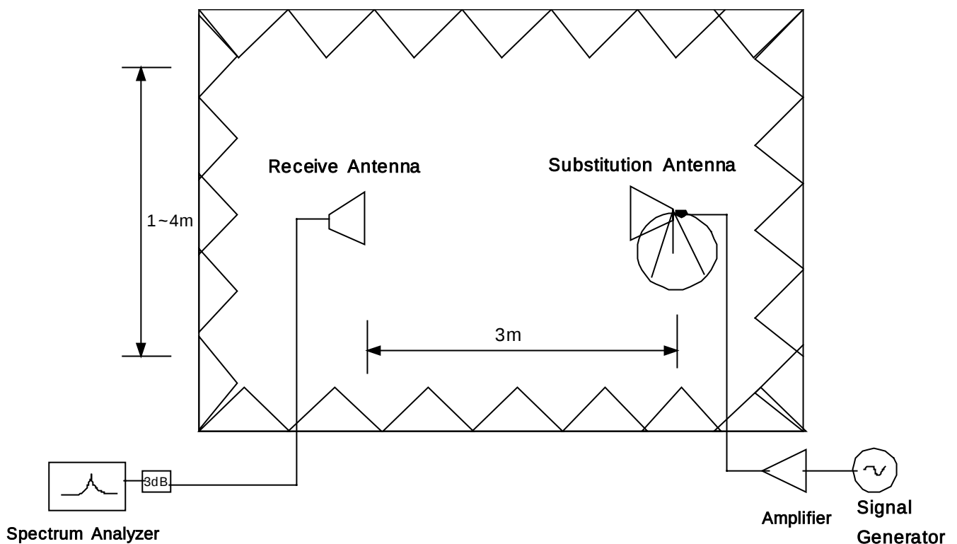
Figure 3. Diagram of EIRP test Set-up
