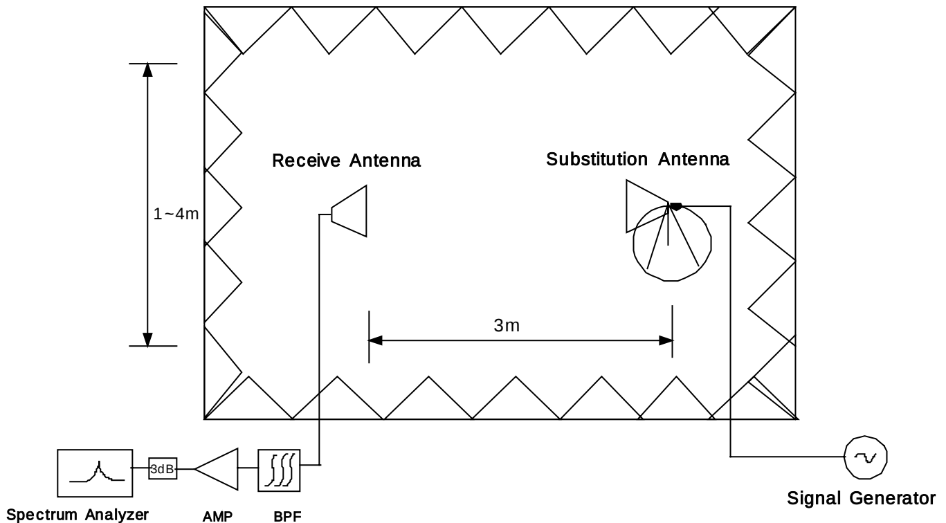
Figure 4. Diagram of Radiated Spurious & Harmonic test Set-up
