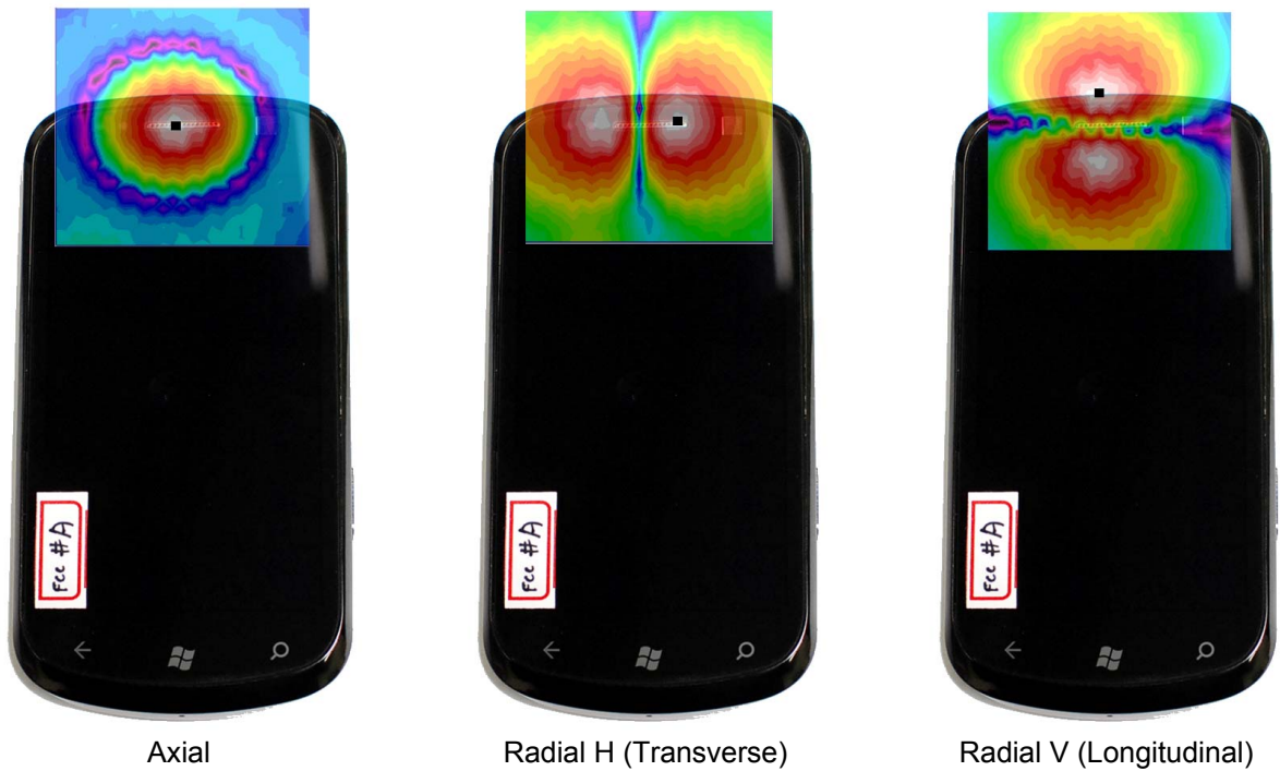
Figure 13-3 T-Coil Scan Overlay Magnetic Field Distributions
