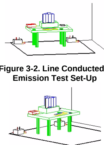
Figure 3-2. Line Conducted Emission Test Set-Up
