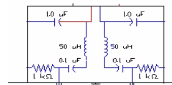
Figure 3-3. Wooden Table & Bonded LISNs
