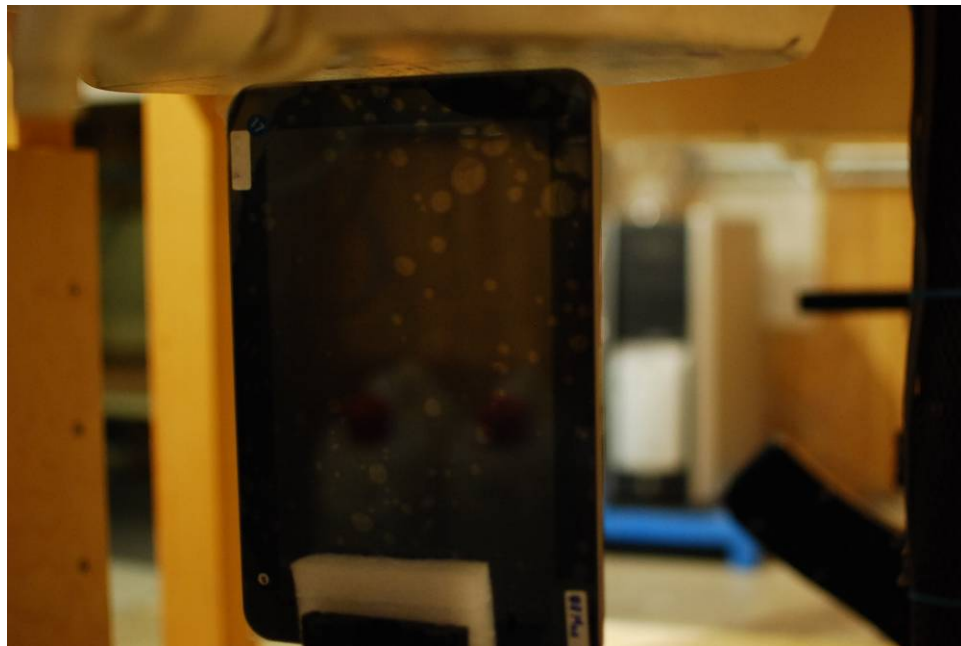
SAR Test Setup Photo 6: Left at 0.5 cm
