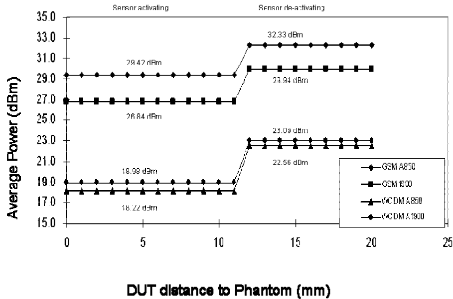
Figure 15-1 Back Off Sensor Power Reduction Graph
