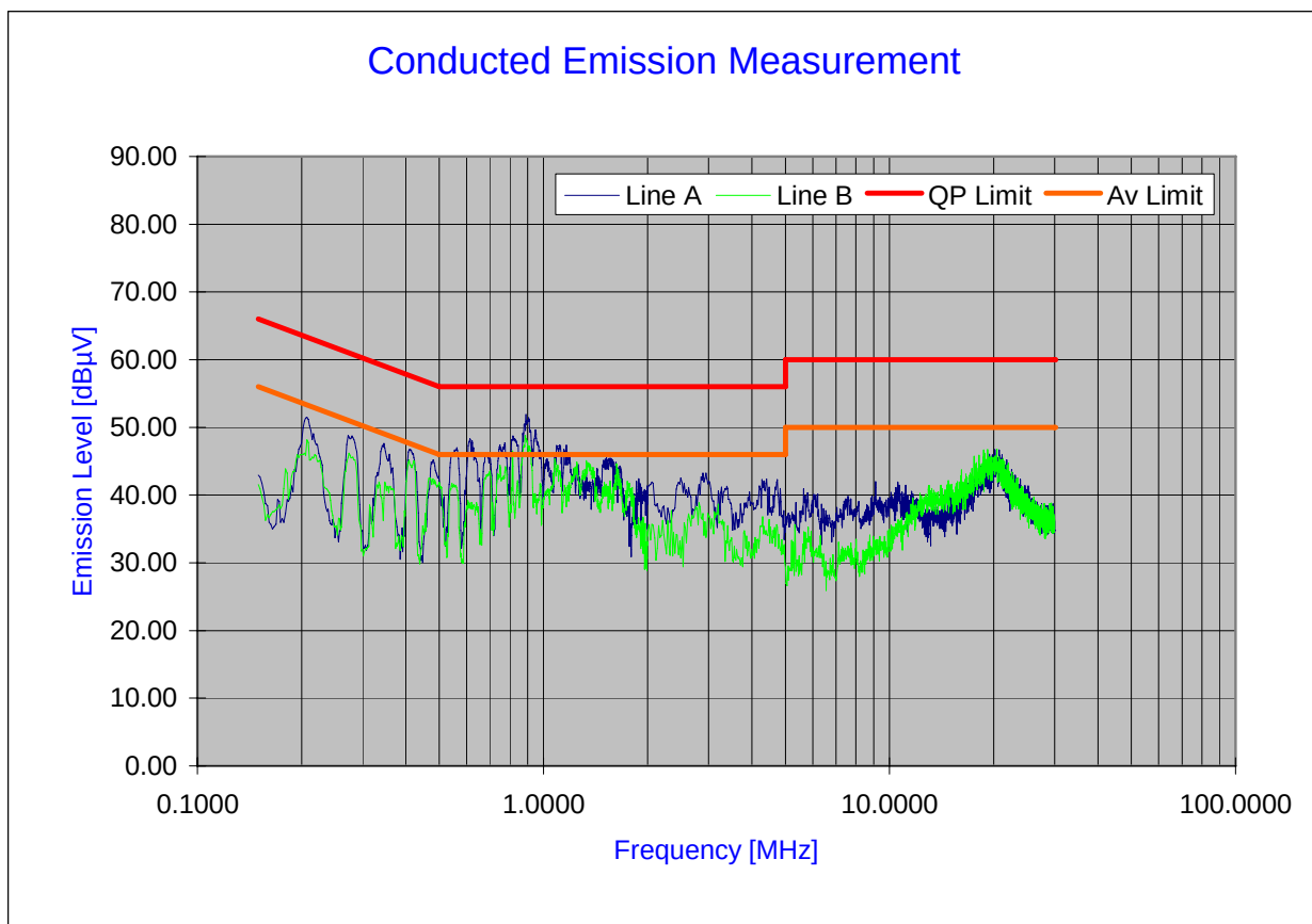
Plot 6-21. Line Conducted Plot with 802.11n
