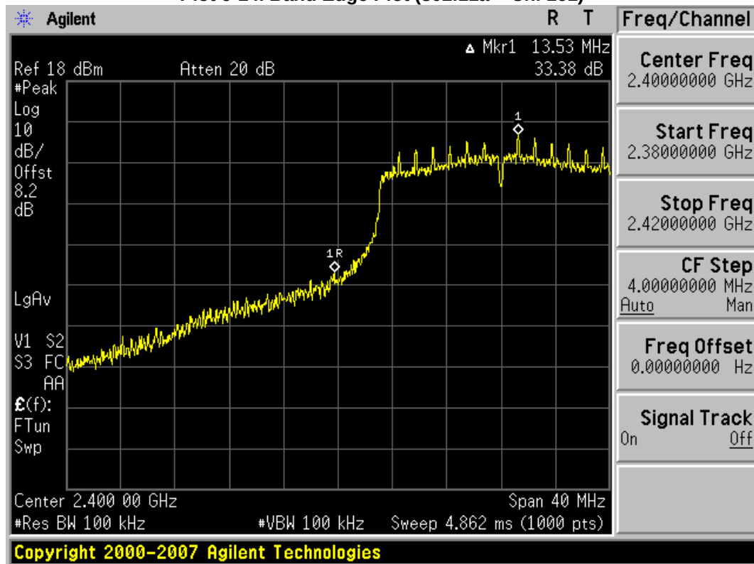
Plot 6-15. Band Edge Plot (802.11n (2.4GHz) – Ch. 1)
