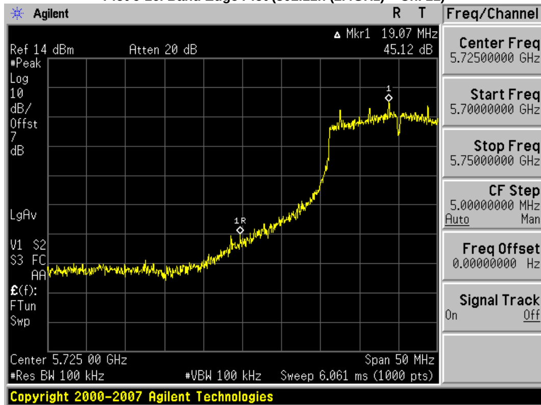
Plot 6-17. Band Edge Plot (802.11n (5.8GHz) – Ch. 149)
