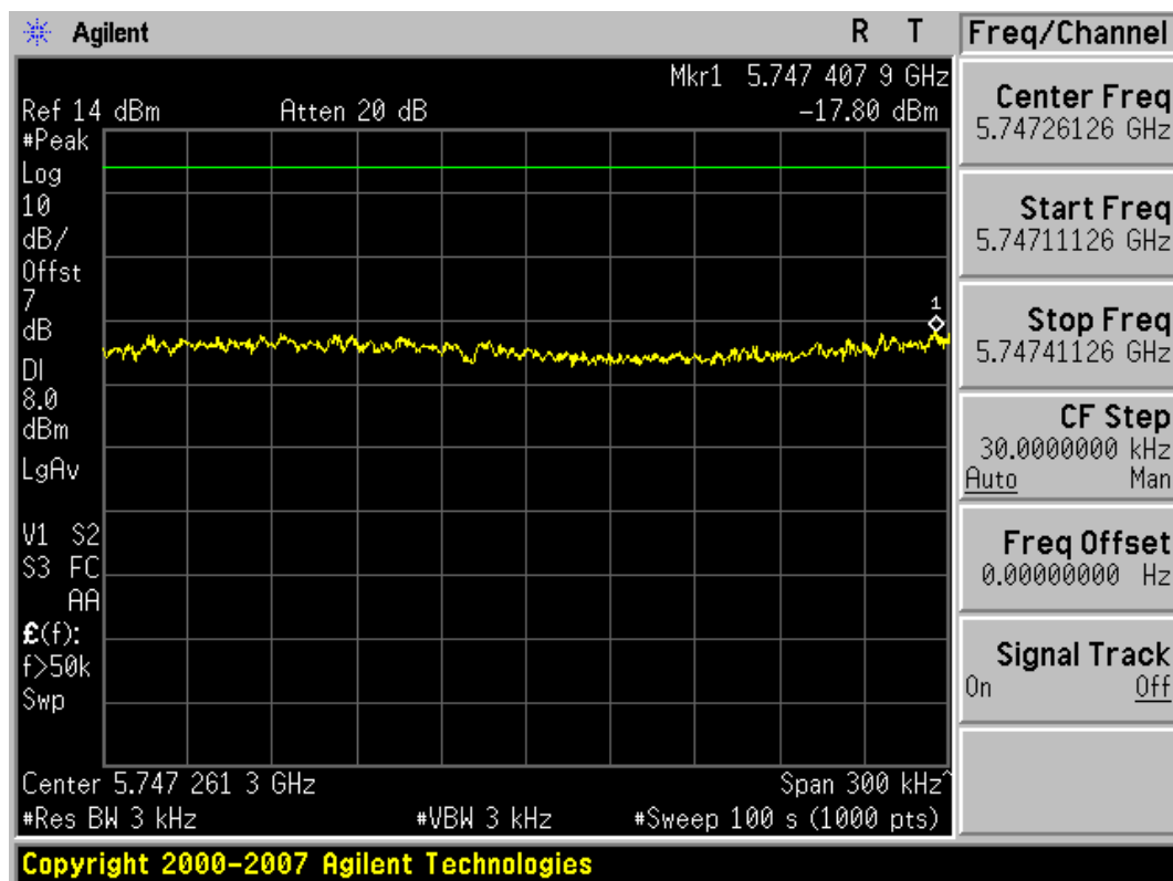
Plot 6-7. Power Spectral Density Plot (802.11a – Ch. 149)
