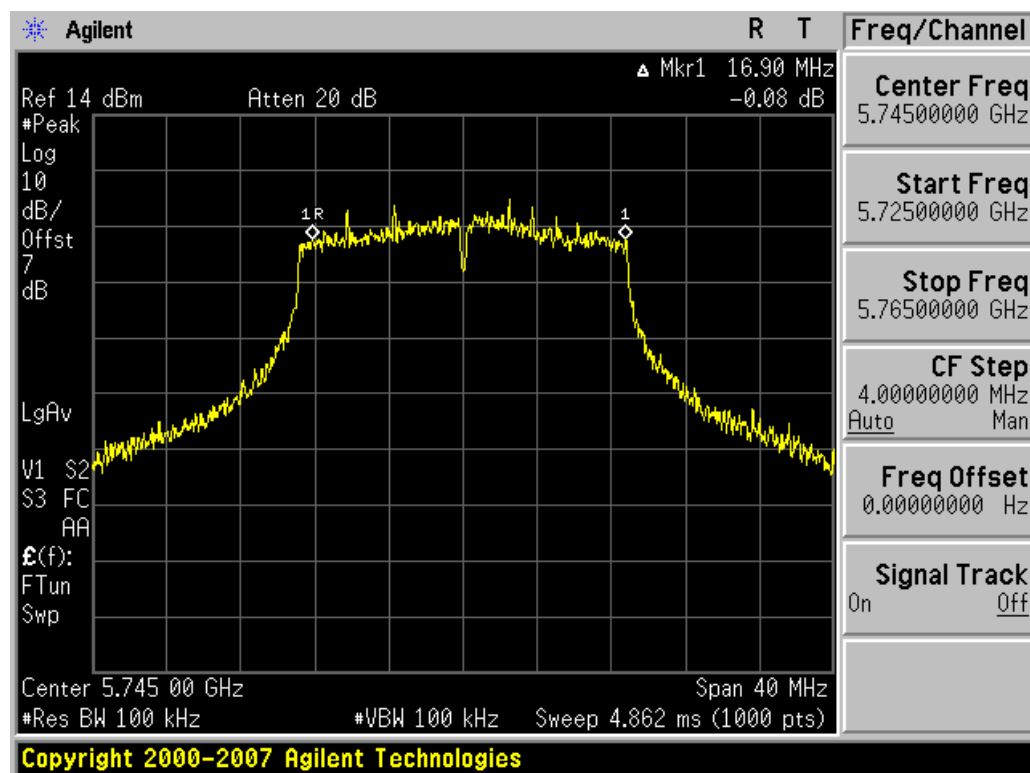
Plot 6-4. 6dB Bandwidth Plot (802.11n (5.8GHz) – Ch. 149)
