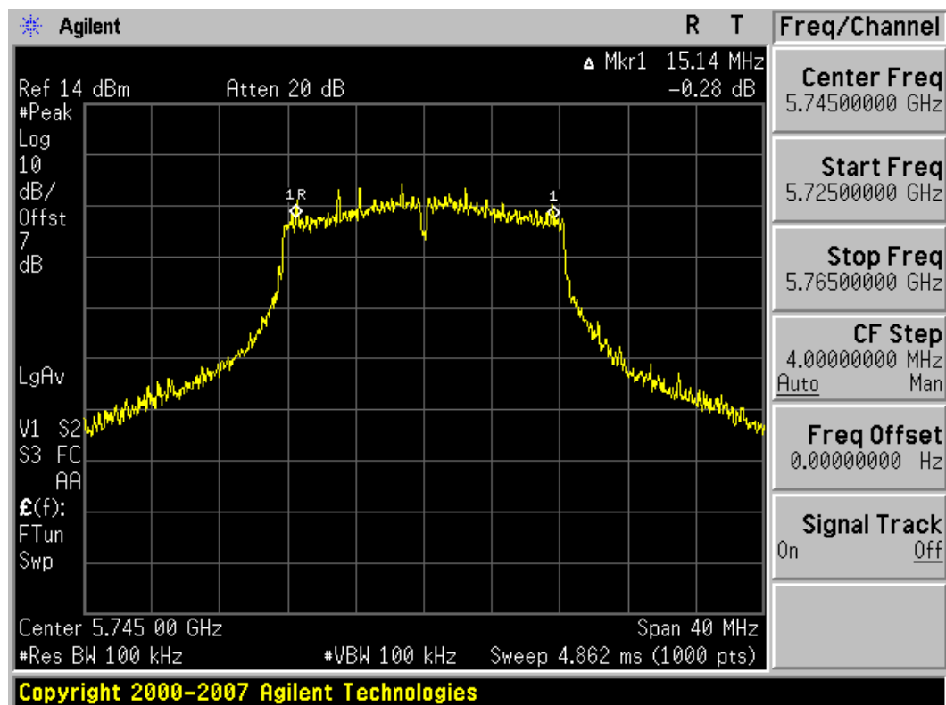
Plot 6-1. 6dB Bandwidth Plot (802.11a – Ch. 149)
