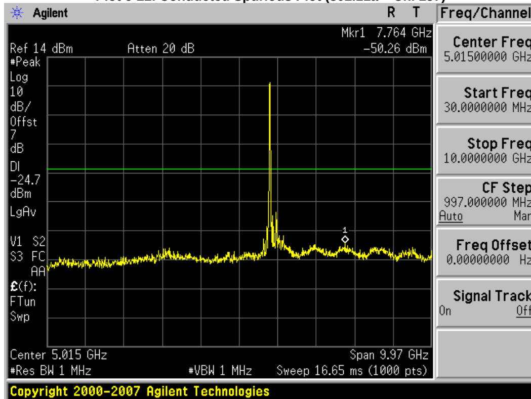
Plot 6-23. Conducted Spurious Plot (802.11a – Ch. 161)
