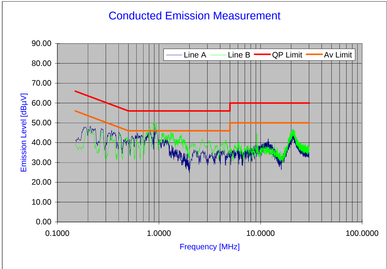
Plot 6-26. Line Conducted Plot with 802.11n
