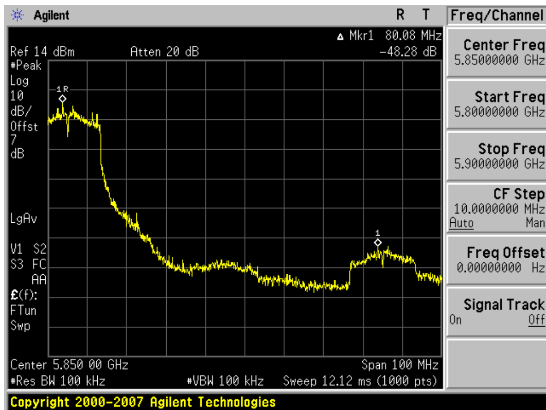
Plot 6-14. Band Edge Plot (802.11a – Ch. 161)
