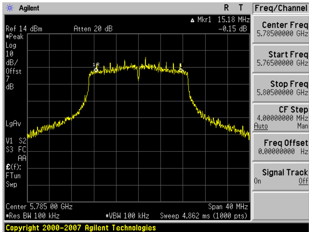
Plot 6-5. 6dB Bandwidth Plot (802.11n (5.8GHz) – Ch. 157)
