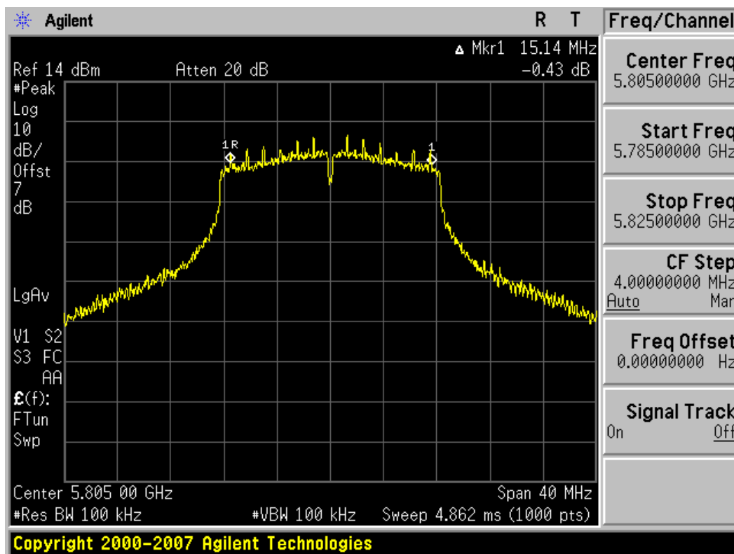
Plot 6-3. 6dB Bandwidth Plot (802.11a – Ch. 161)
