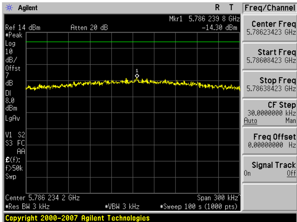
Plot 6-11. Power Spectral Density Plot (802.11n (5.8GHz) – Ch. 157)
