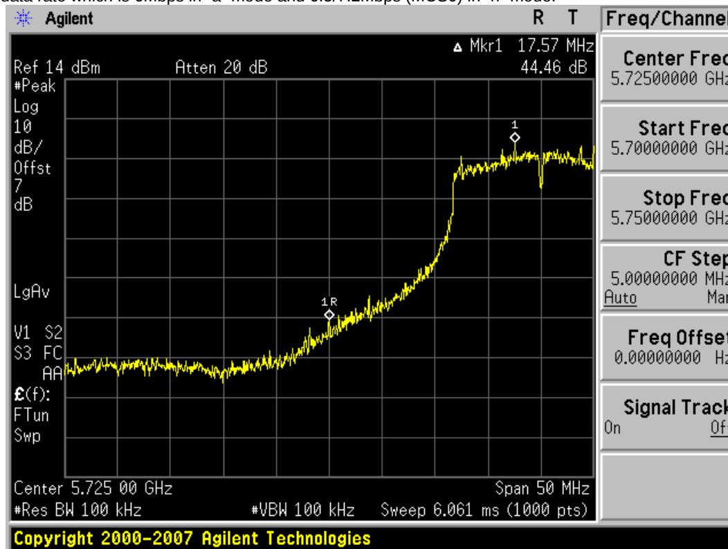
Plot 6-13. Band Edge Plot (802.11a – Ch. 149)
