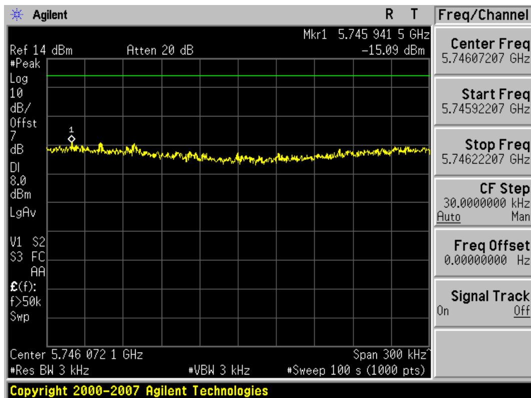
Plot 6-10. Power Spectral Density Plot (802.11n (5.8GHz) – Ch. 149)
