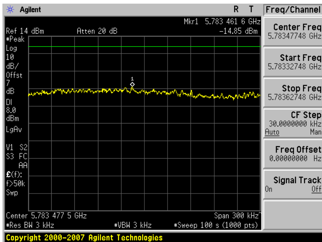
Plot 6-8. Power Spectral Density Plot (802.11a – Ch. 157)
