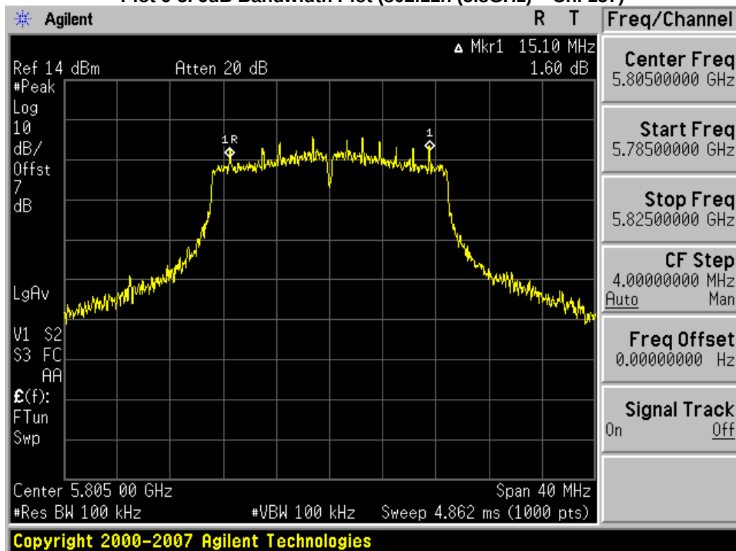
Plot 6-6. 6dB Bandwidth Plot (802.11n (5.8GHz) – Ch. 161)
