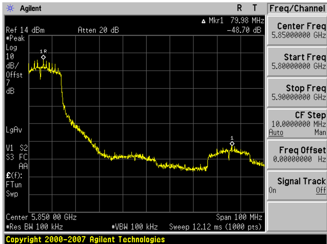
Plot 6-18. Band Edge Plot (802.11n (5.8GHz) – Ch. 161)
