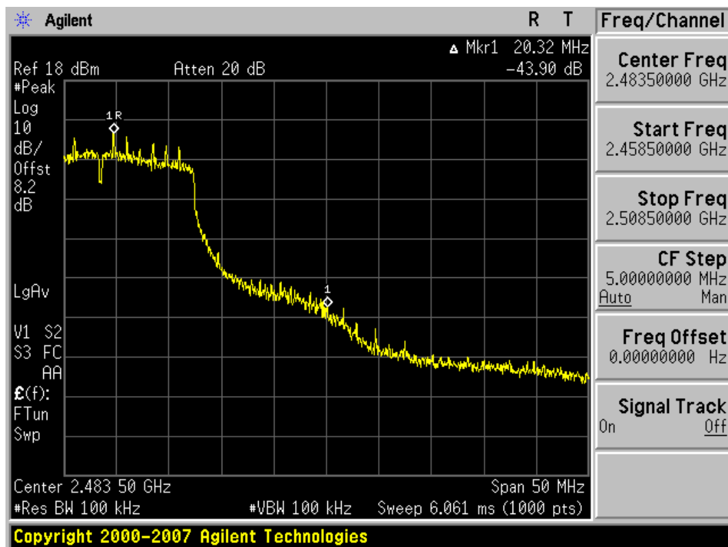
Plot 6-16. Band Edge Plot (802.11n (2.4GHz) – Ch. 11)
