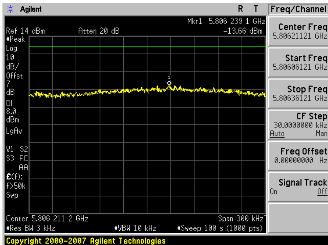
Plot 6-12. Power Spectral Density Plot (802.11n (5.8GHz) – Ch. 161)
