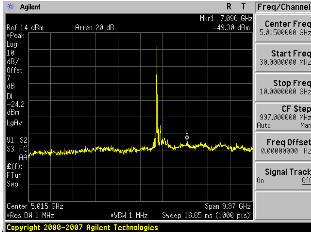
Plot 6-19. Conducted Spurious Plot (802.11a – Ch. 149)
