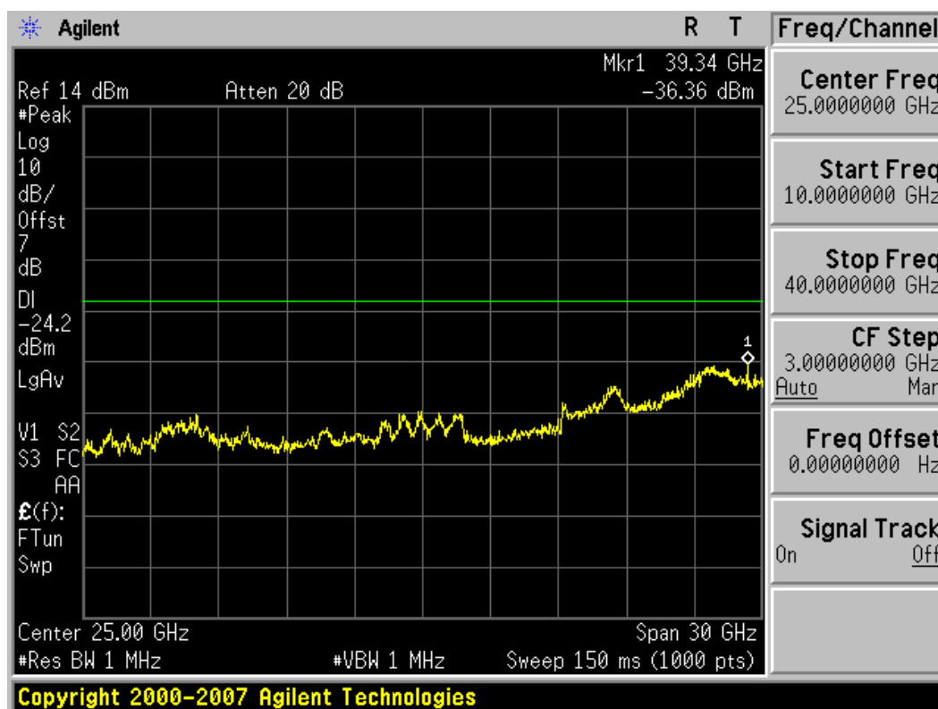
Plot 6-20. Conducted Spurious Plot (802.11a – Ch. 149)
