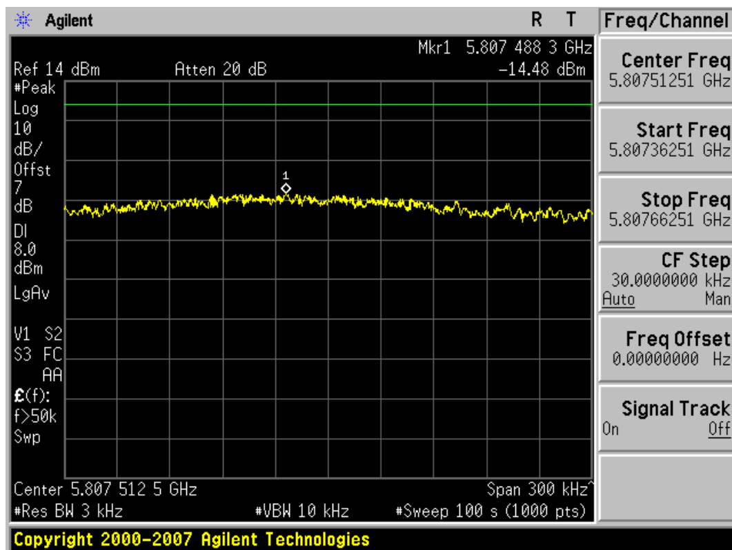
Plot 6-9. Power Spectral Density Plot (802.11a – Ch. 161)
