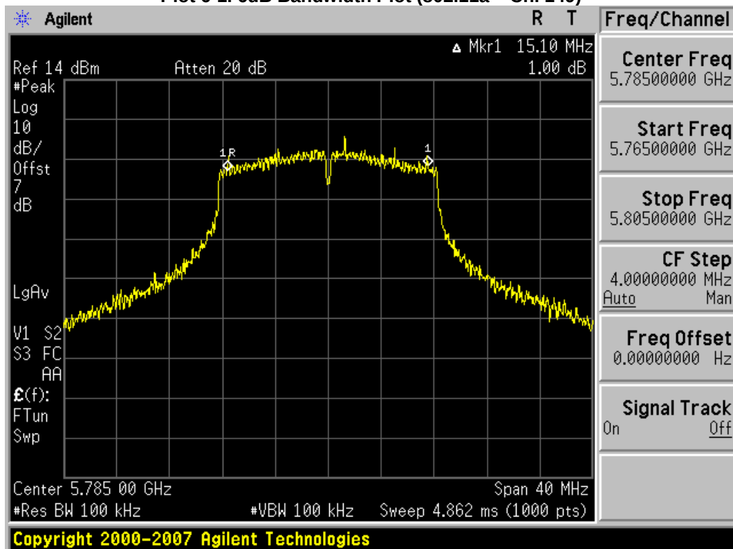
Plot 6-2. 6dB Bandwidth Plot (802.11a – Ch. 157)
