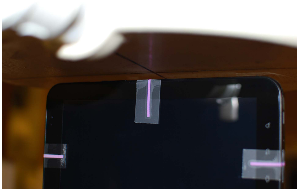
Figure 20-6 SAR Test Setup Photo 5 – Right at 0.5 cm
