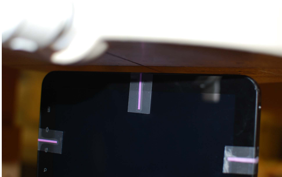
Figure 20-5 SAR Test Setup Photo 4 – Left at 0.5 cm
