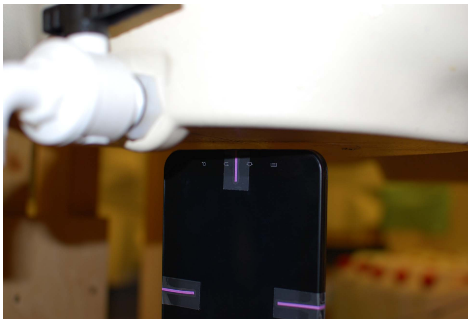
Figure 20-4 SAR Test Setup Photo 3 – Bottom at 0.5 cm
