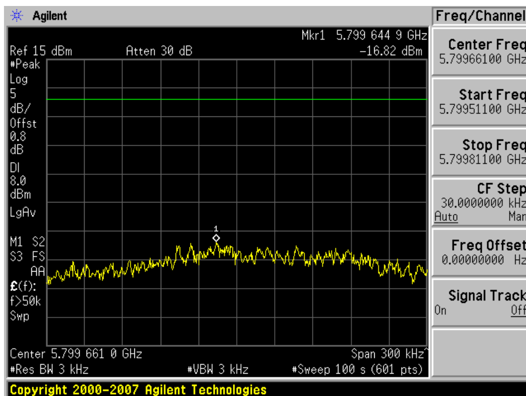
Plot 6-28. Power Spectral Density Plot (802.11n (5.8GHz) – Ch. 161)
