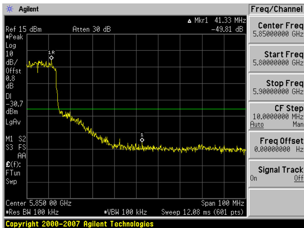
Plot 6-34. Band Edge Plot (802.11a – Ch. 161)
