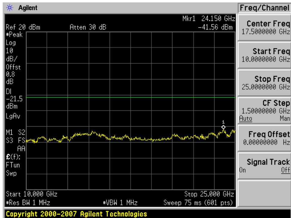
Plot 6-40. Conducted Spurious Plot (802.11b – Ch. 1)
