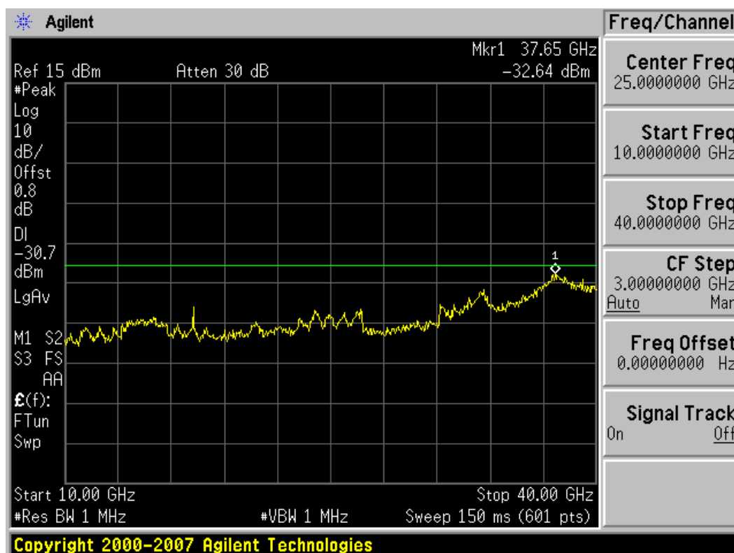
Plot 6-50. Conducted Spurious Plot (802.11a – Ch. 161)
