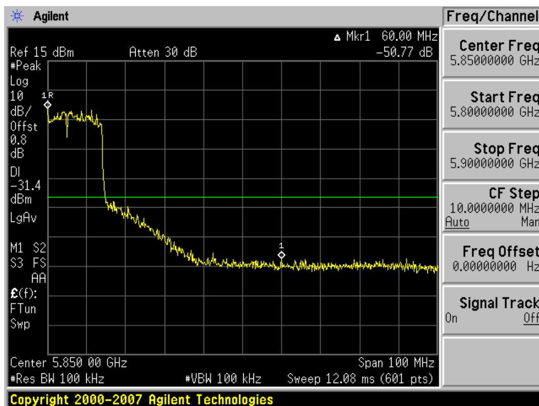
Plot 6-38. Band Edge Plot (802.11n (5.8GHz) – Ch. 161)
