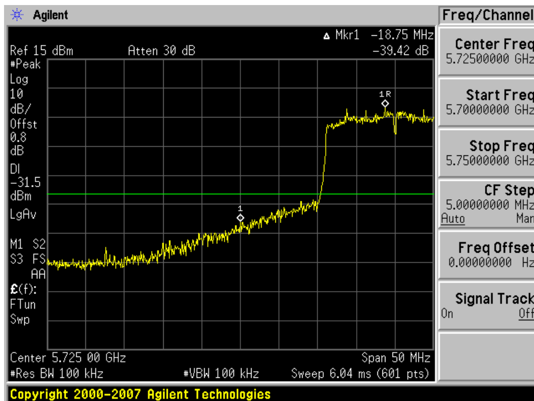
Plot 6-37. Band Edge Plot (802.11n (5.8GHz) – Ch. 149)
