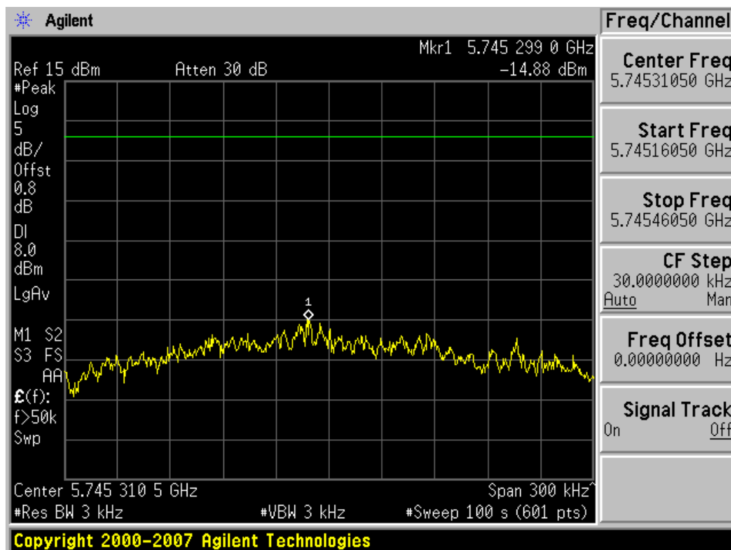
Plot 6-27. Power Spectral Density Plot (802.11n (5.8GHz) – Ch. 149)
