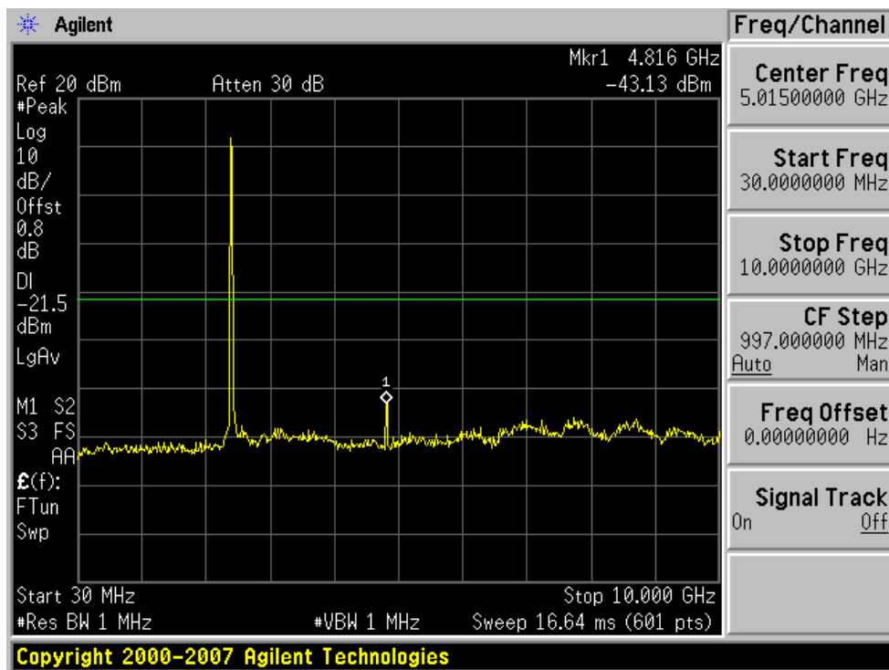
Plot 6-39. Conducted Spurious Plot (802.11b – Ch. 1)
