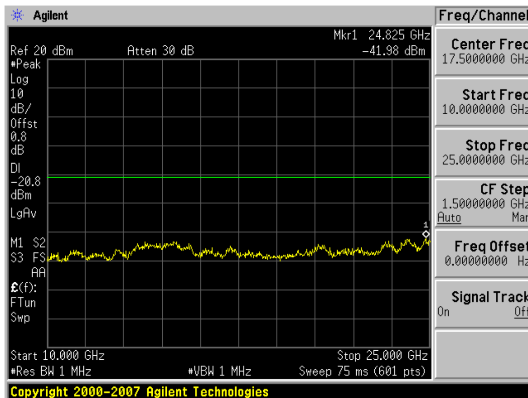
Plot 6-42. Conducted Spurious Plot (802.11b – Ch. 6)
