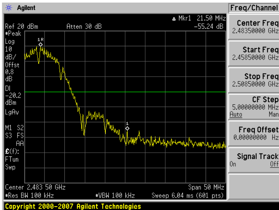
Plot 6-30. Band Edge Plot (802.11b – Ch. 11)
