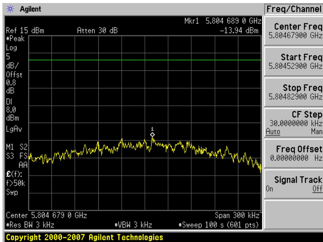
Plot 6-23. Power Spectral Density Plot (802.11a – Ch. 161)
