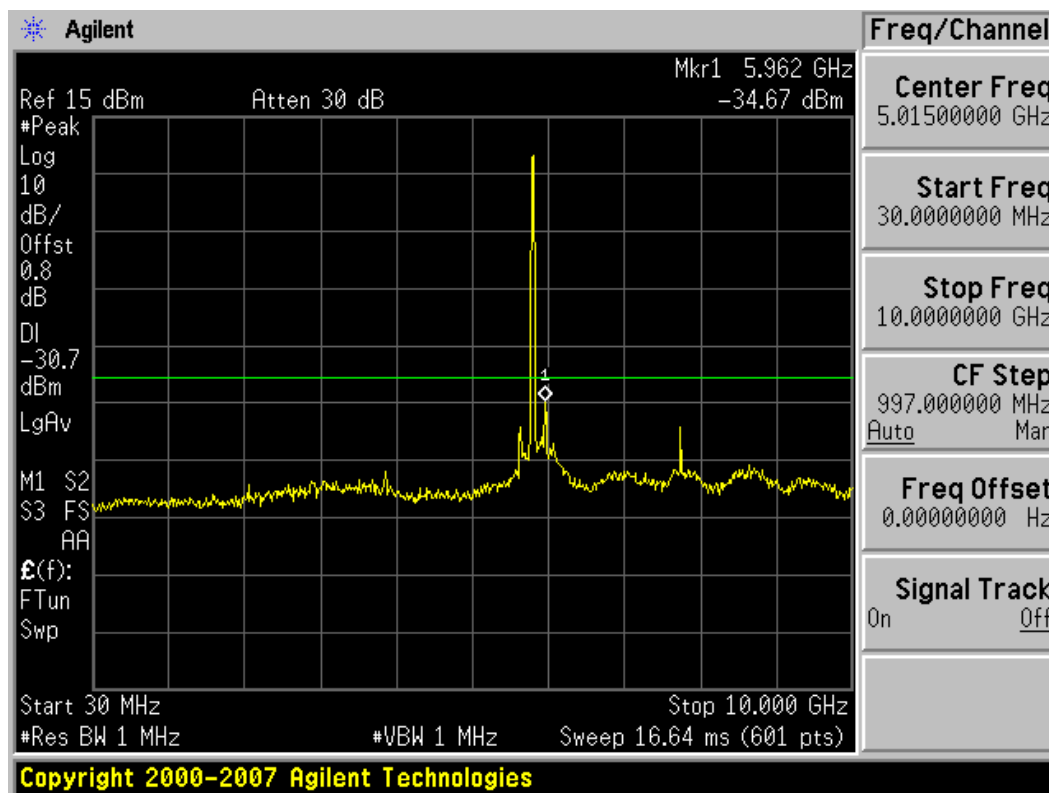
Plot 6-49. Conducted Spurious Plot (802.11a – Ch. 161)
