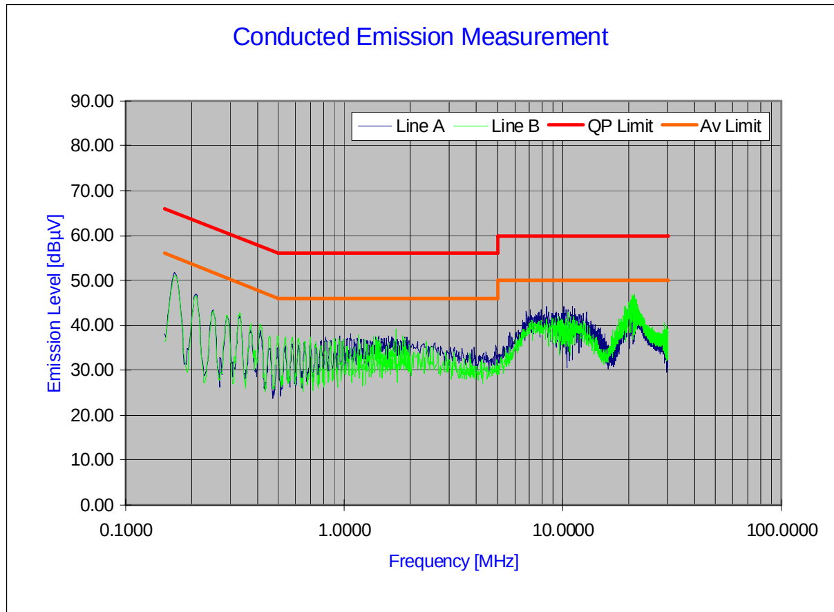
Plot 6-51. Line Conducted Plot with 802.11b
