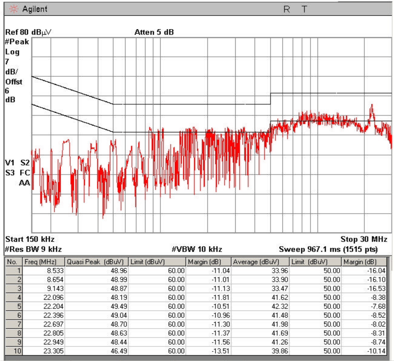
Plot 7-1. Line-Conducted Test Plot
