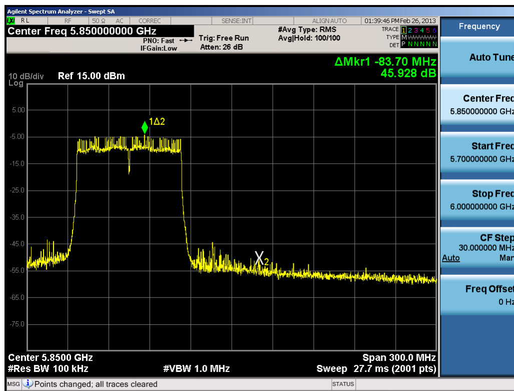
Plot 6-50. Band Edge Plot (80MHz BW 802.11ac (5.8GHz) – Ch. 155)
