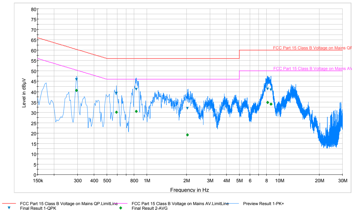
Plot 6-24. Line Conducted Plot with Bluetooth LE (N)
