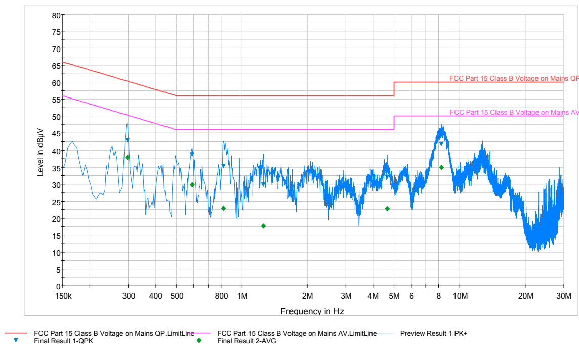
Plot 6-23. Line Conducted Plot with Bluetooth LE (L1)
