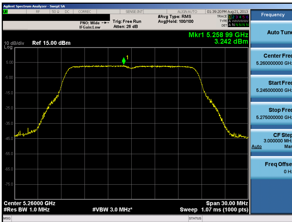
Plot 6-42. Peak Power Spectral Density Plot (802.11a (UNII Band 2) – Ch. 52)
