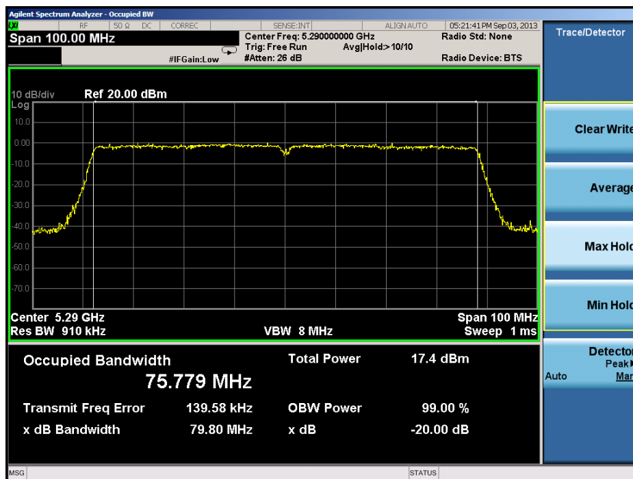
Plot 6-32. 20dB Bandwidth Plot (80MHz BW 802.11ac (UNII Band 2) – Ch. 58)
