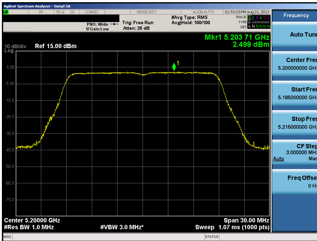
Plot 6-37. Peak Power Spectral Density Plot (20MHz BW 802.11n (UNII Band 1) – Ch. 40)
