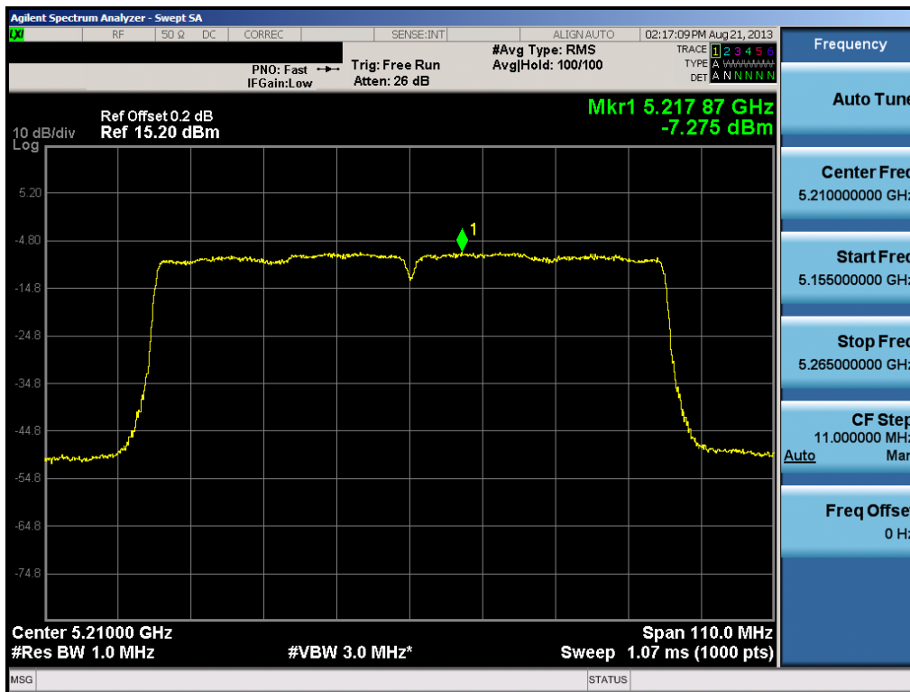
Plot 6-41. Peak Power Spectral Density Plot (80MHz BW 802.11ac (UNII Band 1) – Ch. 42)
