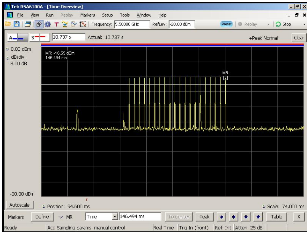
Figure 6-1. Type 1 Radar Pulse
