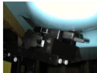
Figure 17. PCS Head SAR Test Setup
