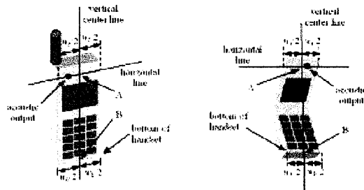
Figure 5.4 Handset vertical and horizontal reference lines
