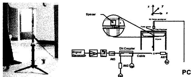
Figure 7.1 Dipole Validation Test Setup
