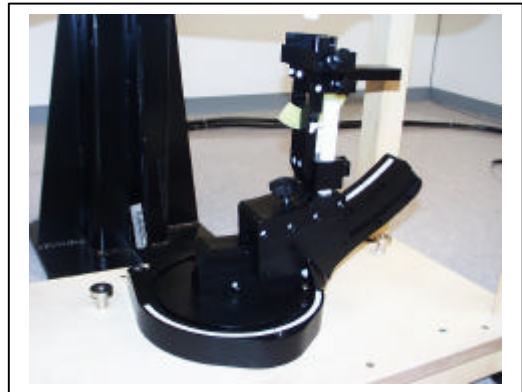
Device Holder
