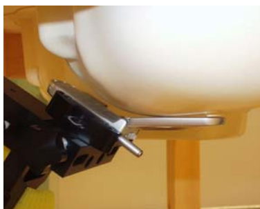
Figure 8.2 Left Head SAR Test Setup
