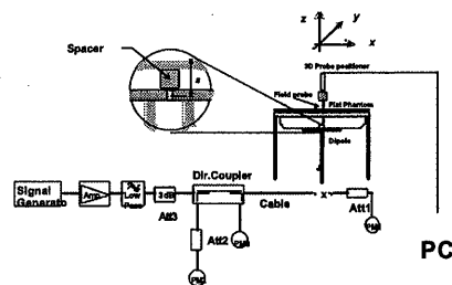
Figure 7.1 Dipole Validation Test Setup
