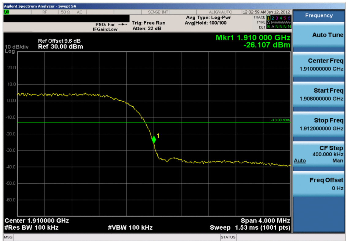
Plot 7-40. Band Edge Plot (PCS WCDMA Mode – Ch. 9538)
