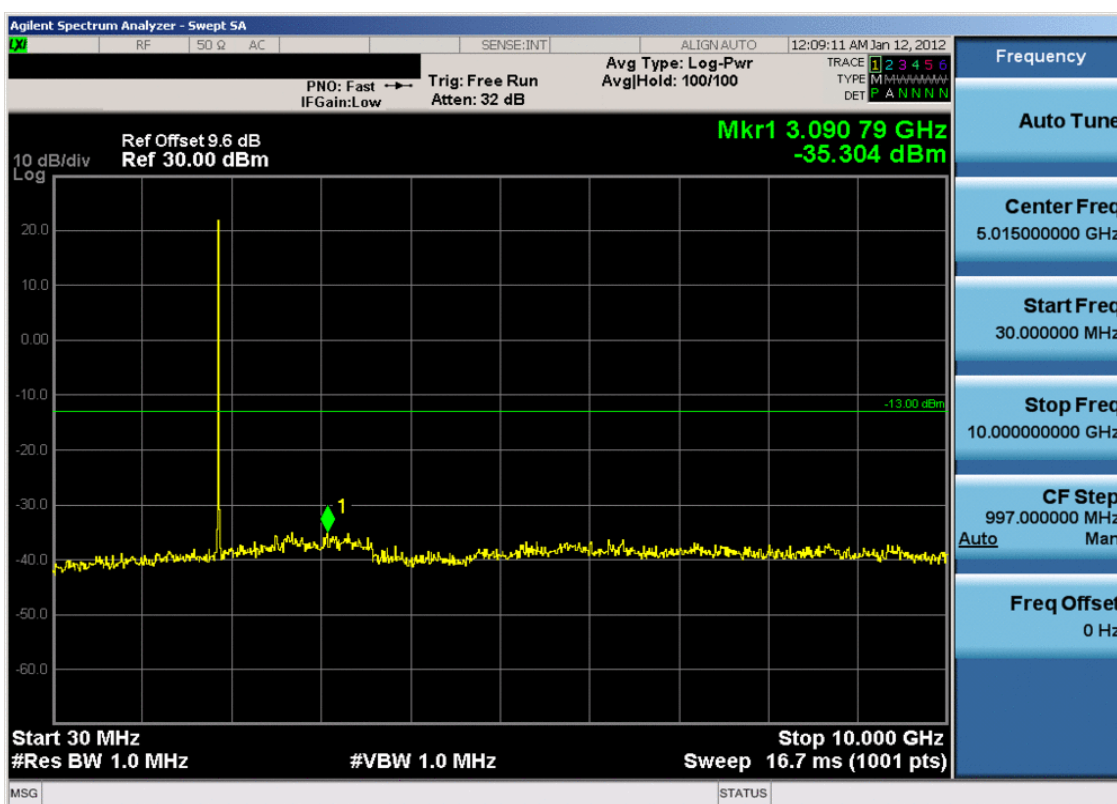
Plot 7-34. Conducted Spurious Plot (PCS WCDMA Mode – Ch. 9400)
