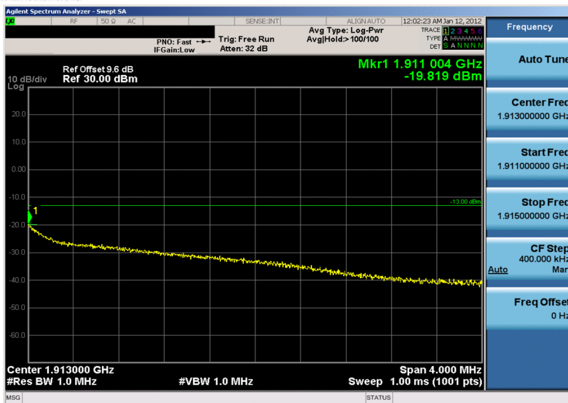
Plot 7-41. 4MHz Span Plot (PCS WCDMA Mode – Ch. 9538)
