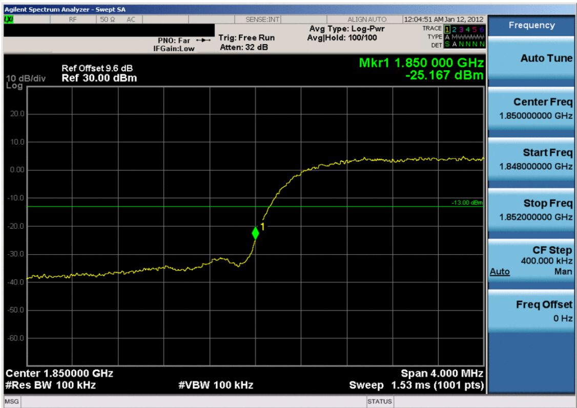
Plot 7-32. Band Edge Plot (PCS WCDMA Mode – Ch. 9262)
