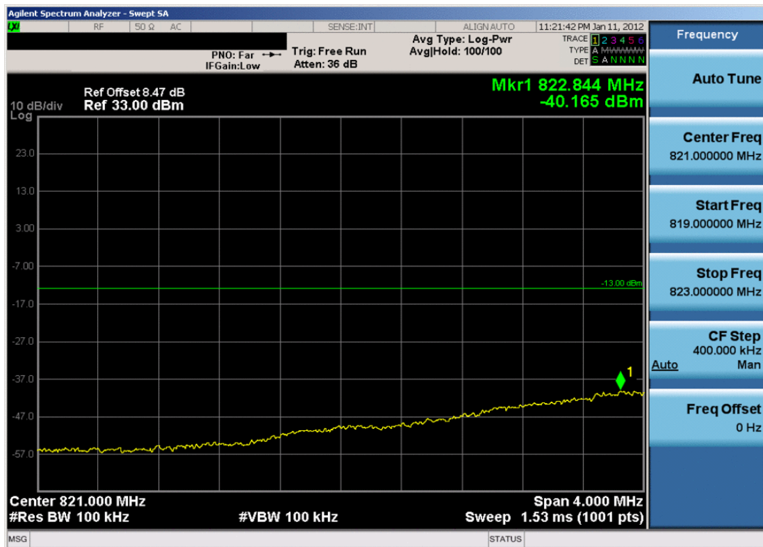
Plot 7-22. 4MHz Span Plot (Cellular WCDMA Mode – Ch. 4132)
