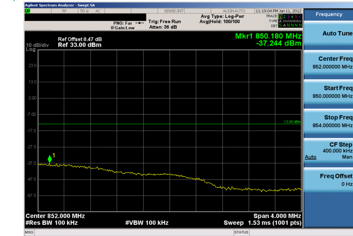
Plot 7-29. 4MHz Span Plot (Cellular WCDMA Mode – Ch. 4233)
