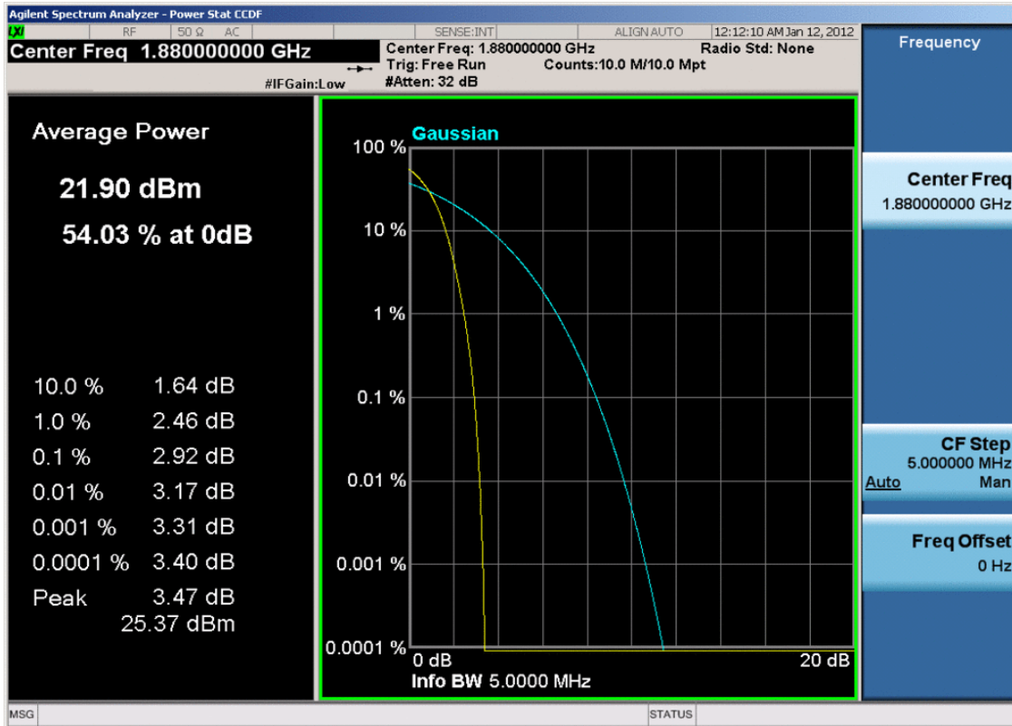
Plot 7-37. Peak-Average Ratio Plot (PCS WCDMA Mode – Ch. 9400)
