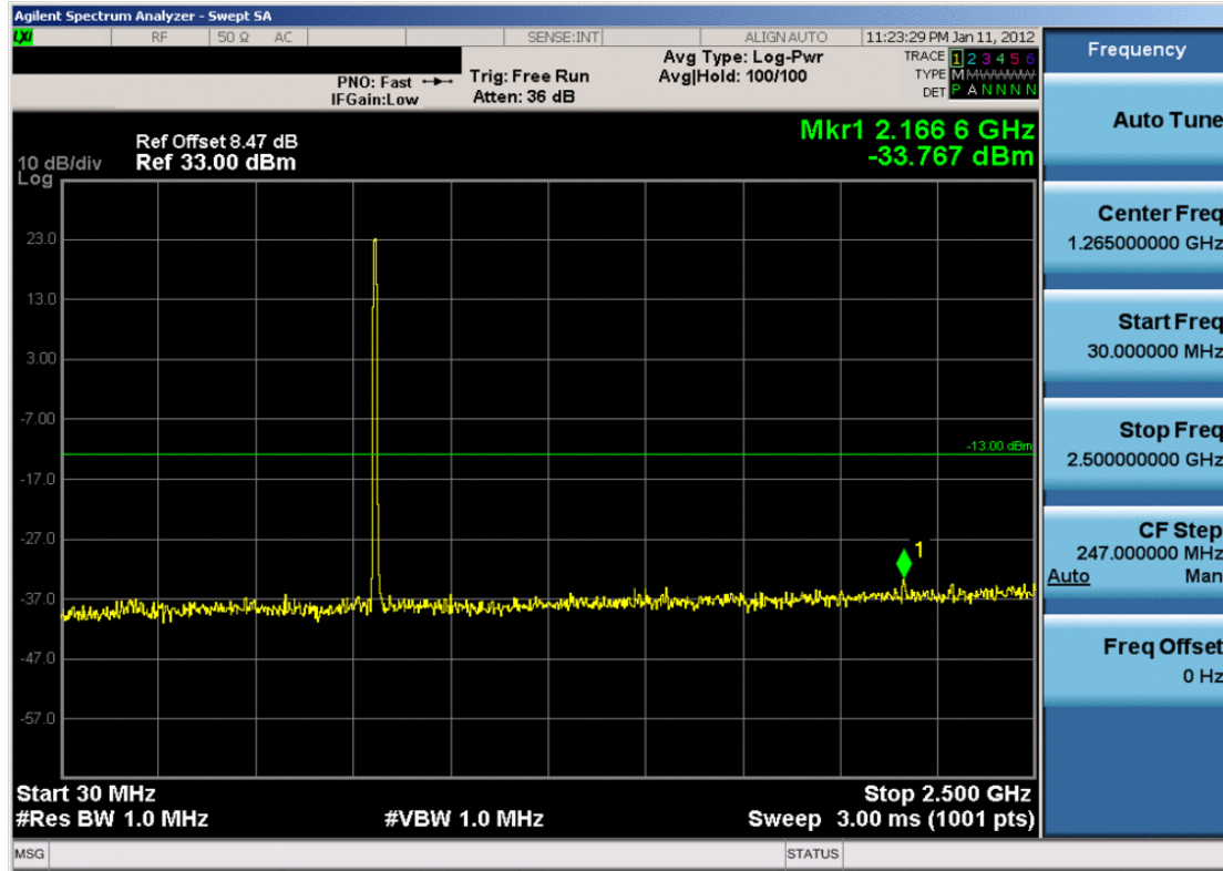
Plot 7-19. Conducted Spurious Plot (Cellular WCDMA Mode – Ch. 4132)
