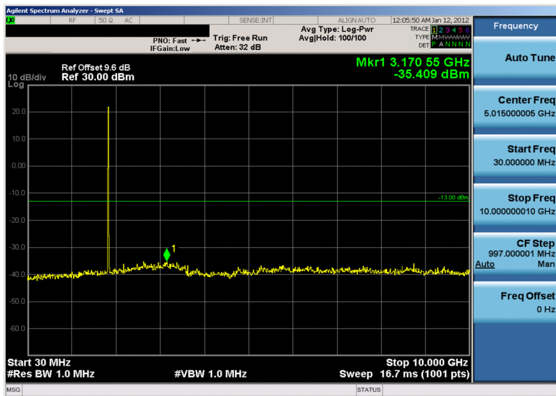
Plot 7-30. Conducted Spurious Plot (PCS WCDMA Mode – Ch. 9262)
