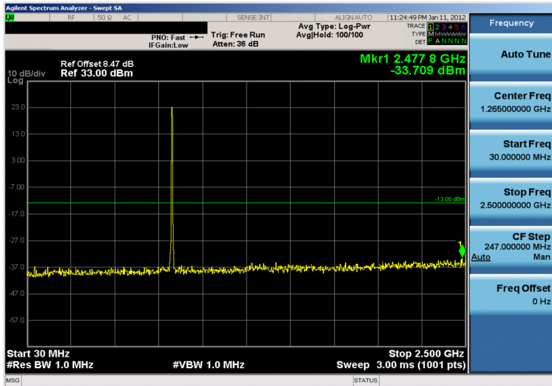
Plot 7-26. Conducted Spurious Plot (Cellular WCDMA Mode – Ch. 4233)
