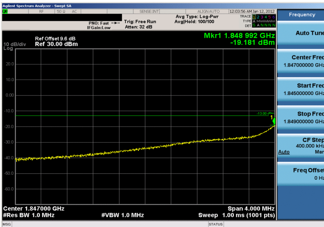
Plot 7-33. 4MHz Span Plot (PCS WCDMA Mode – Ch. 9262)
