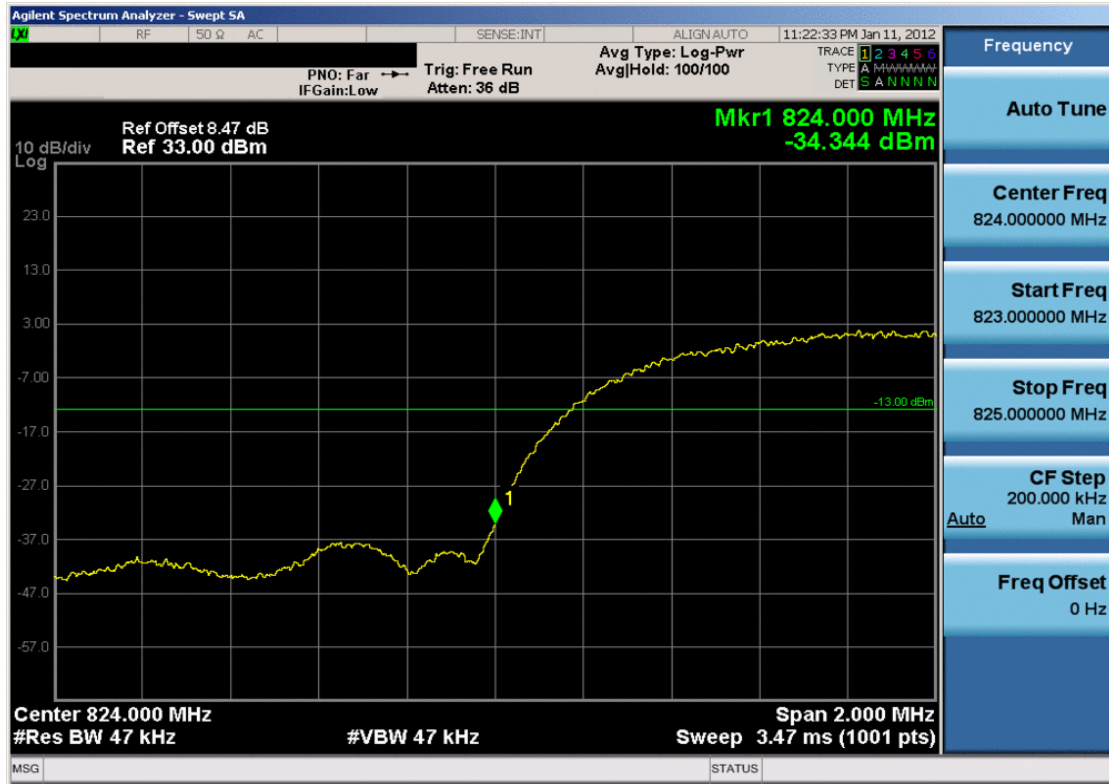
Plot 7-21. Band Edge Plot (Cellular WCDMA Mode – Ch. 4132)
