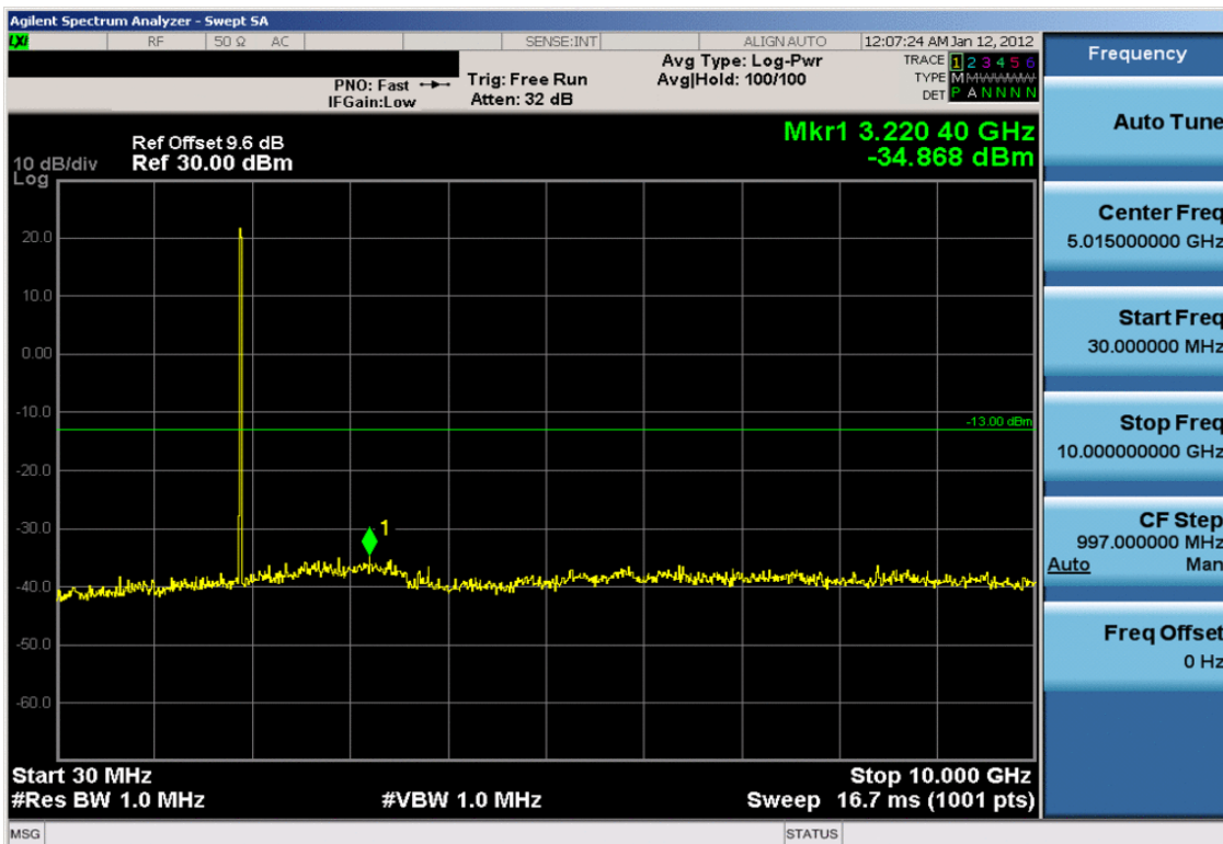
Plot 7-38. Conducted Spurious Plot (PCS WCDMA Mode – Ch. 9538)
