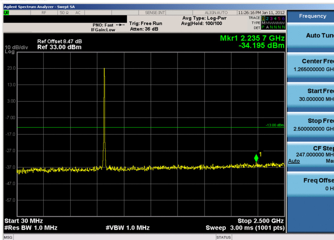
Plot 7-23. Conducted Spurious Plot (Cellular WCDMA Mode – Ch. 4183)
