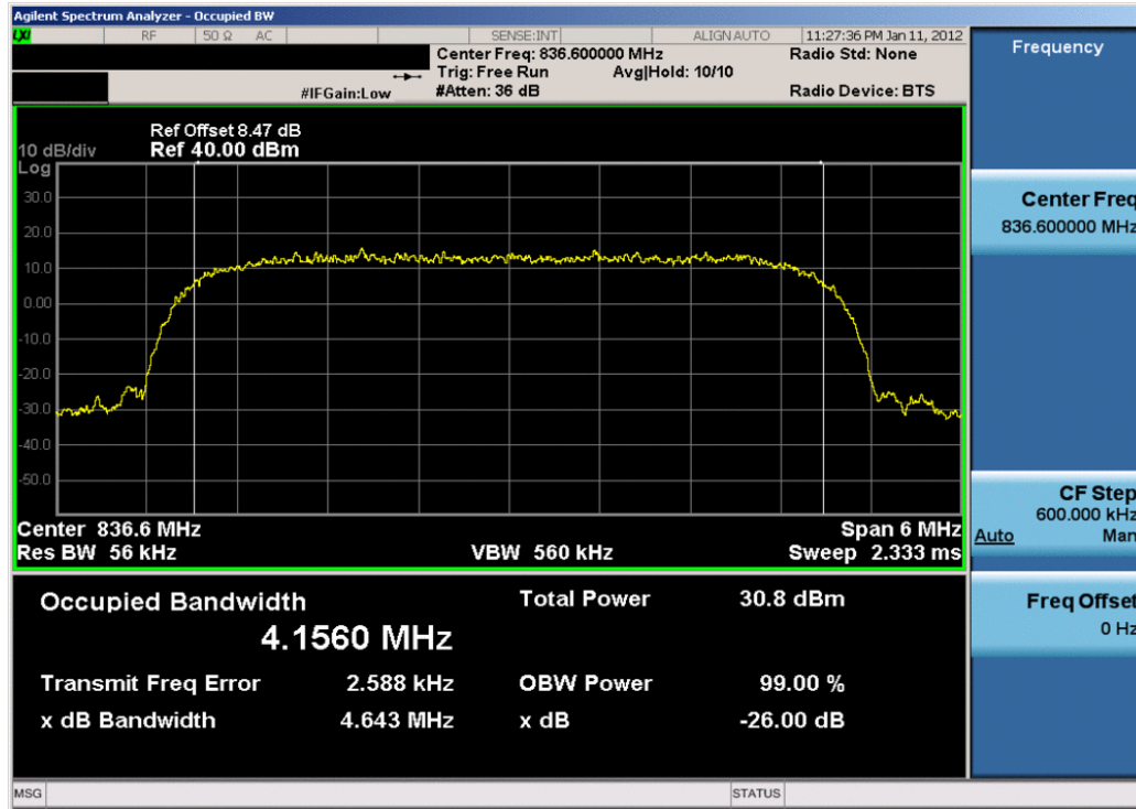
Plot 7-25. Occupied Bandwidth Plot (Cellular WCDMA Mode – Ch. 4183)
