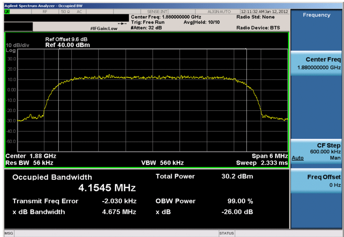
Plot 7-36. Occupied Bandwidth Plot (PCS WCDMA Mode – Ch. 9400)
