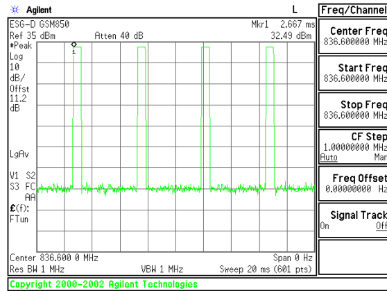
Figure 8-4 GSM850 Signal
