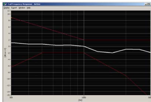
Figure 7-1 Axial Frequency Response
