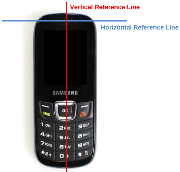
SAR Test Setup Photo 6 – Horizontal and Vertical Reference Lines
