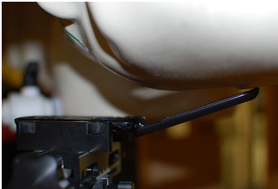
Figure 19-4 SAR Test Setup Photo 4 – Left Tilt
