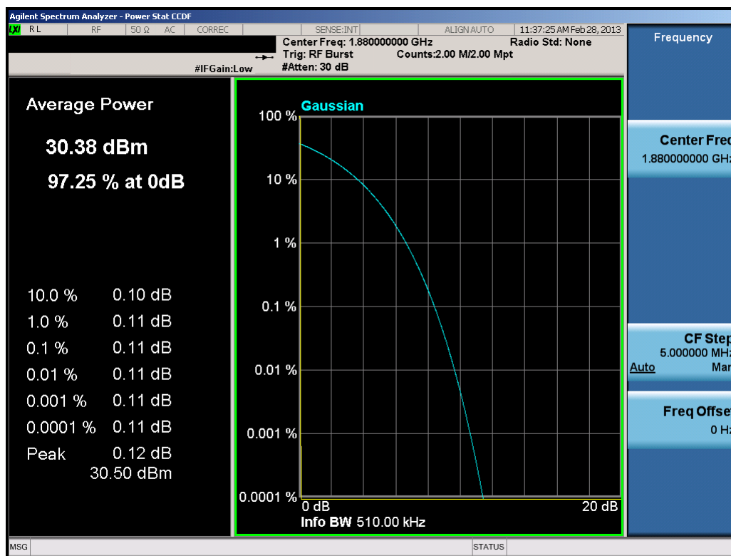
Plot 7-20. Peak-Average Ratio Plot (PCS GSM Mode – Ch. 661)
