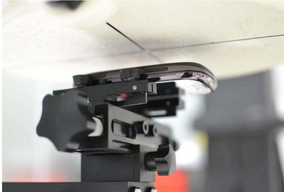
SAR Test Setup Photo 5: Body-Worn at 15 mm
