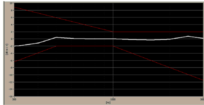
Figure 6-1 Axial Frequency Response
