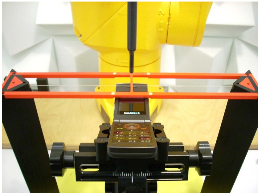
Figure 16-2 HAC Phantom Plane Alignment
