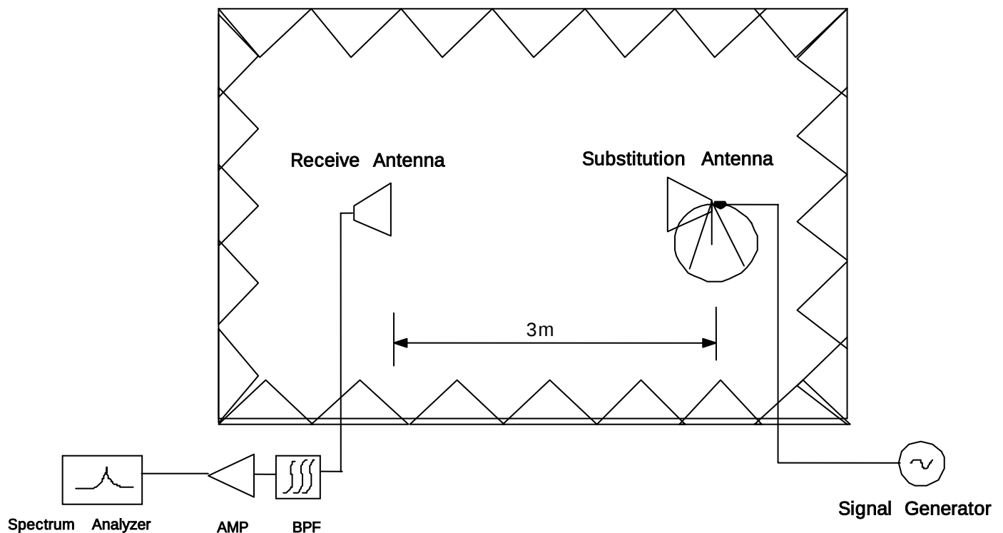
Figure 4. Diagram of Radiated Spurious & Harmonic test Set-up
