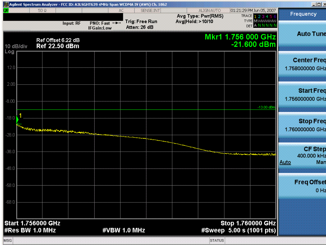
Plot 7-11. 4MHz Span Plot (AWS WCDMA Mode – Ch. 1862)
