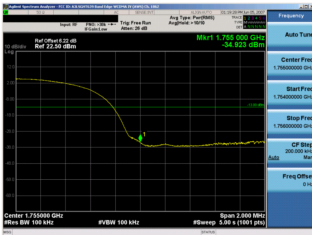
Plot 7-10. Band Edge Plot (AWS WCDMA Mode – Ch. 1862)
