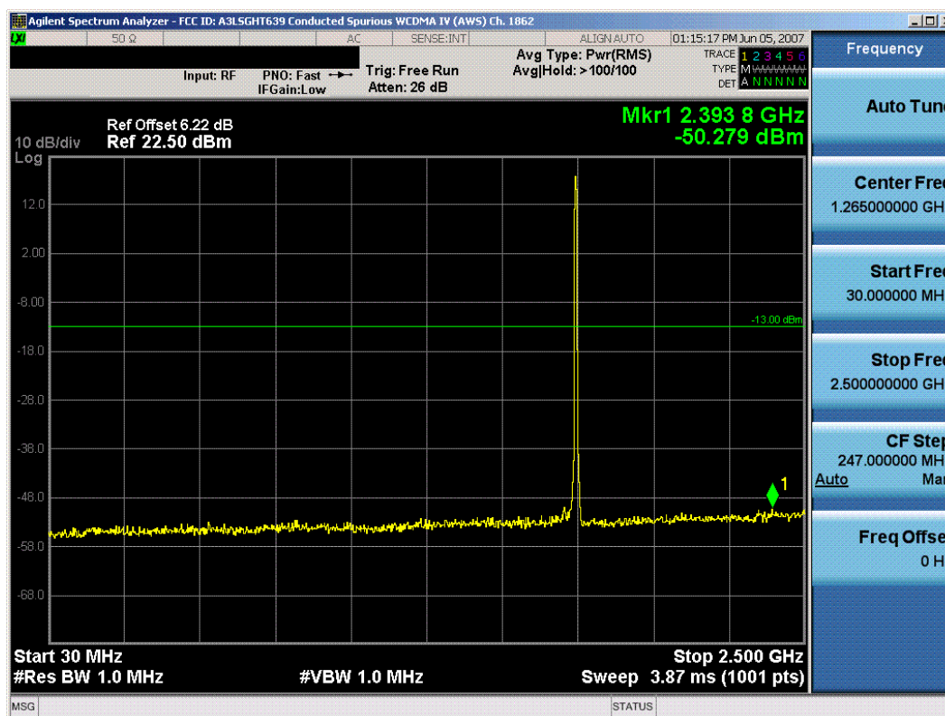
Plot 7-8. Conducted Spurious Plot (AWS WCDMA Mode – Ch. 1862)
