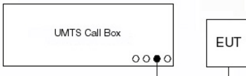
Figure 6-1. WCDMA Conducted Power Test Setup Diagram
