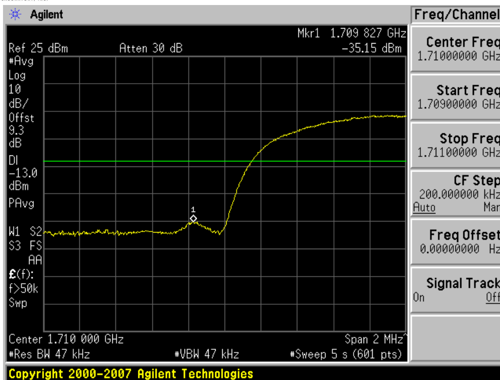
Plot 7-3. Band Edge Plot (AWS WCDMA Mode – Ch. 1312)
