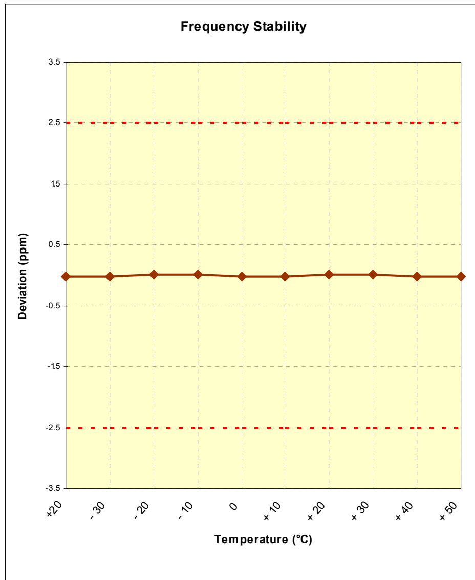
Figure 6-1. Frequency Stability Graph (AWS WCDMA Mode – Ch. 1412)
