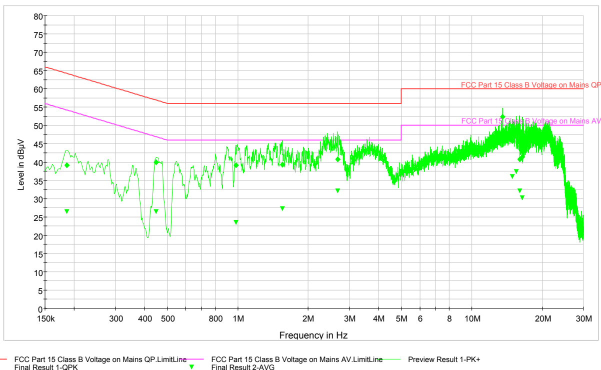
Plot 8-2. Line Conducted Plot (L2)
