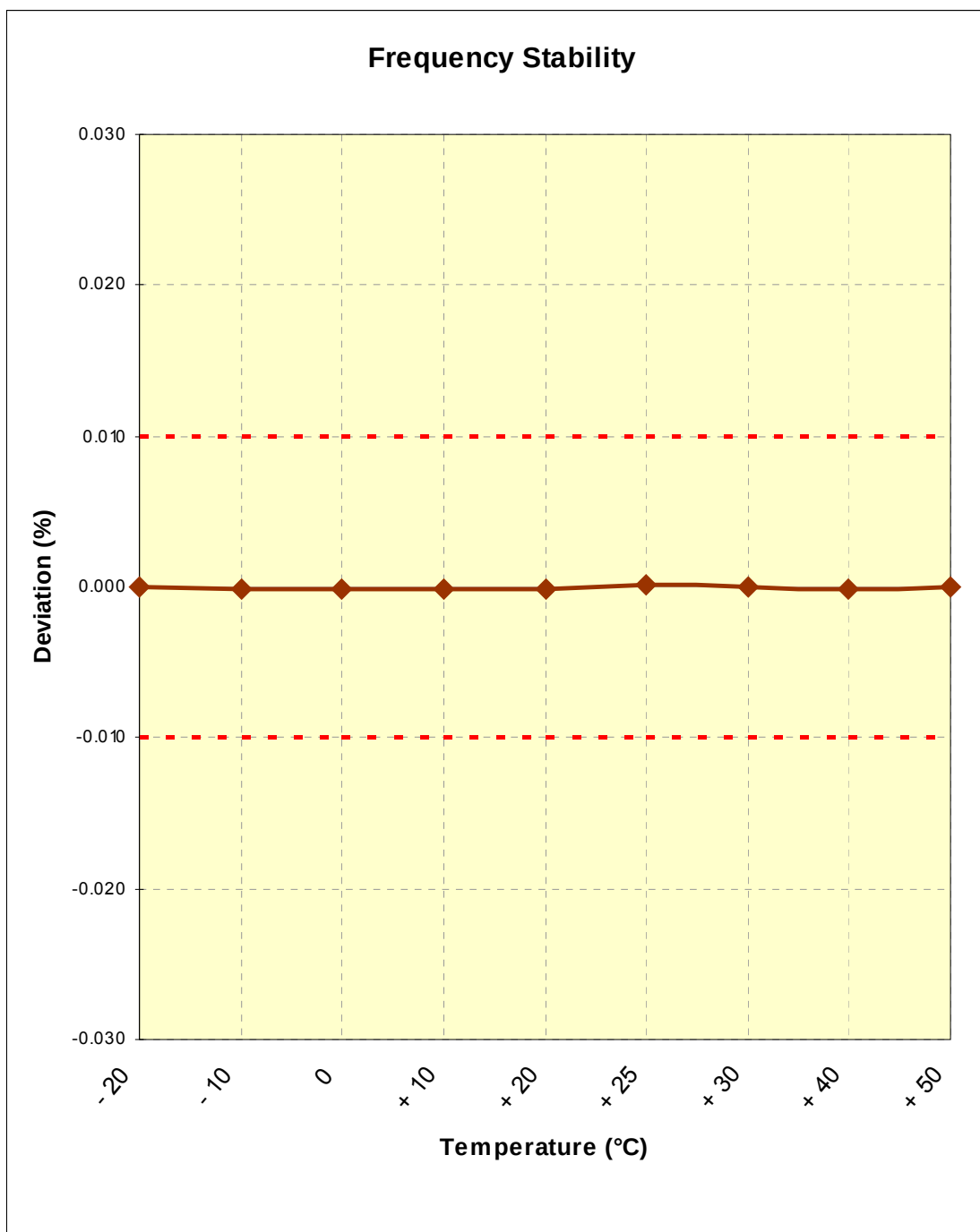
Figure 8-3. Frequency Stability Plot
