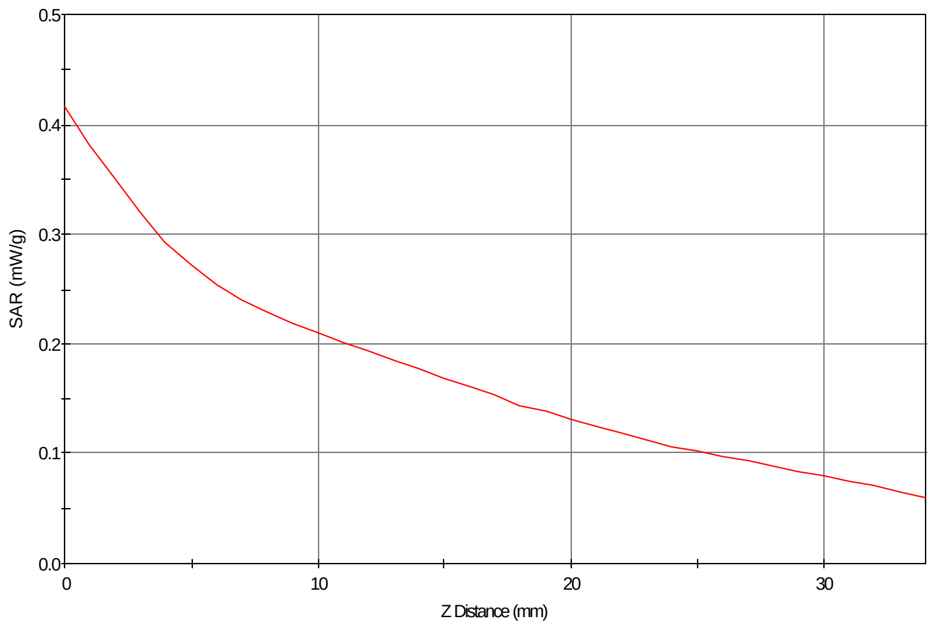
SAR - Z Axis at Hotspot x:37.0 y:11.0
