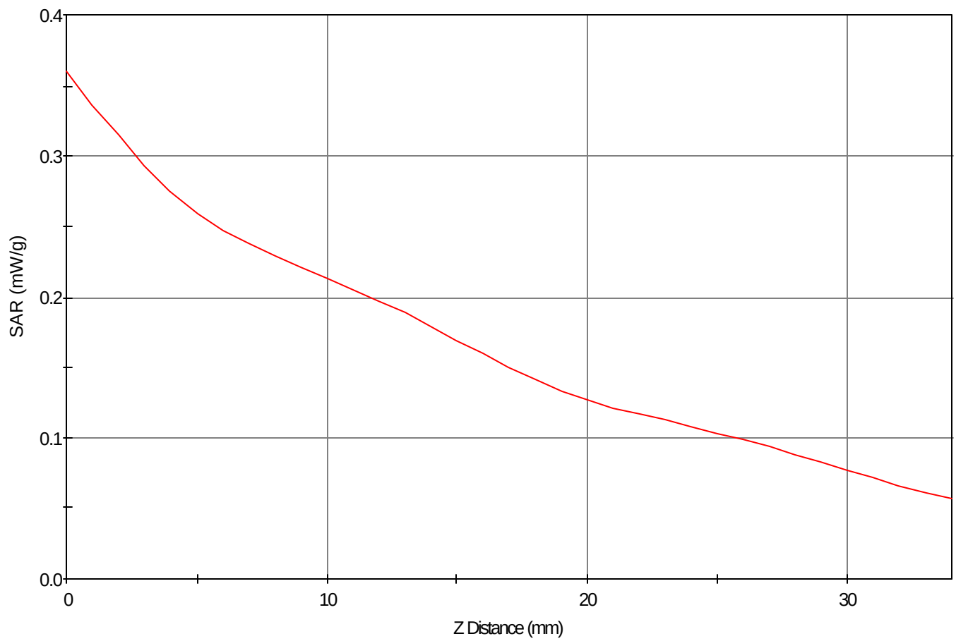
SAR - Z Axis at Hotspot x:47.0 y:9.0
