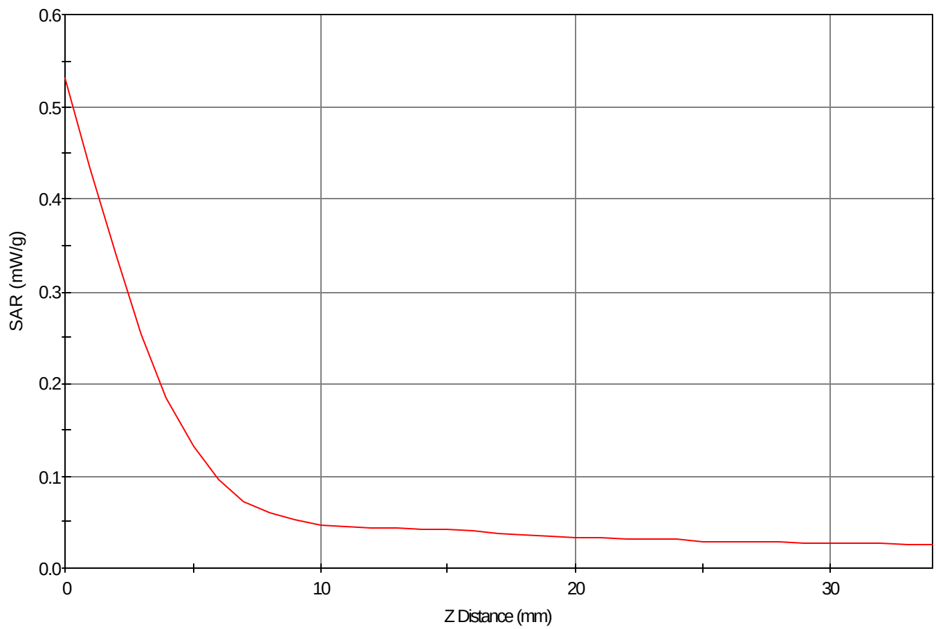
SAR - Z Axis at Hotspot x:14.0 y:12.0
