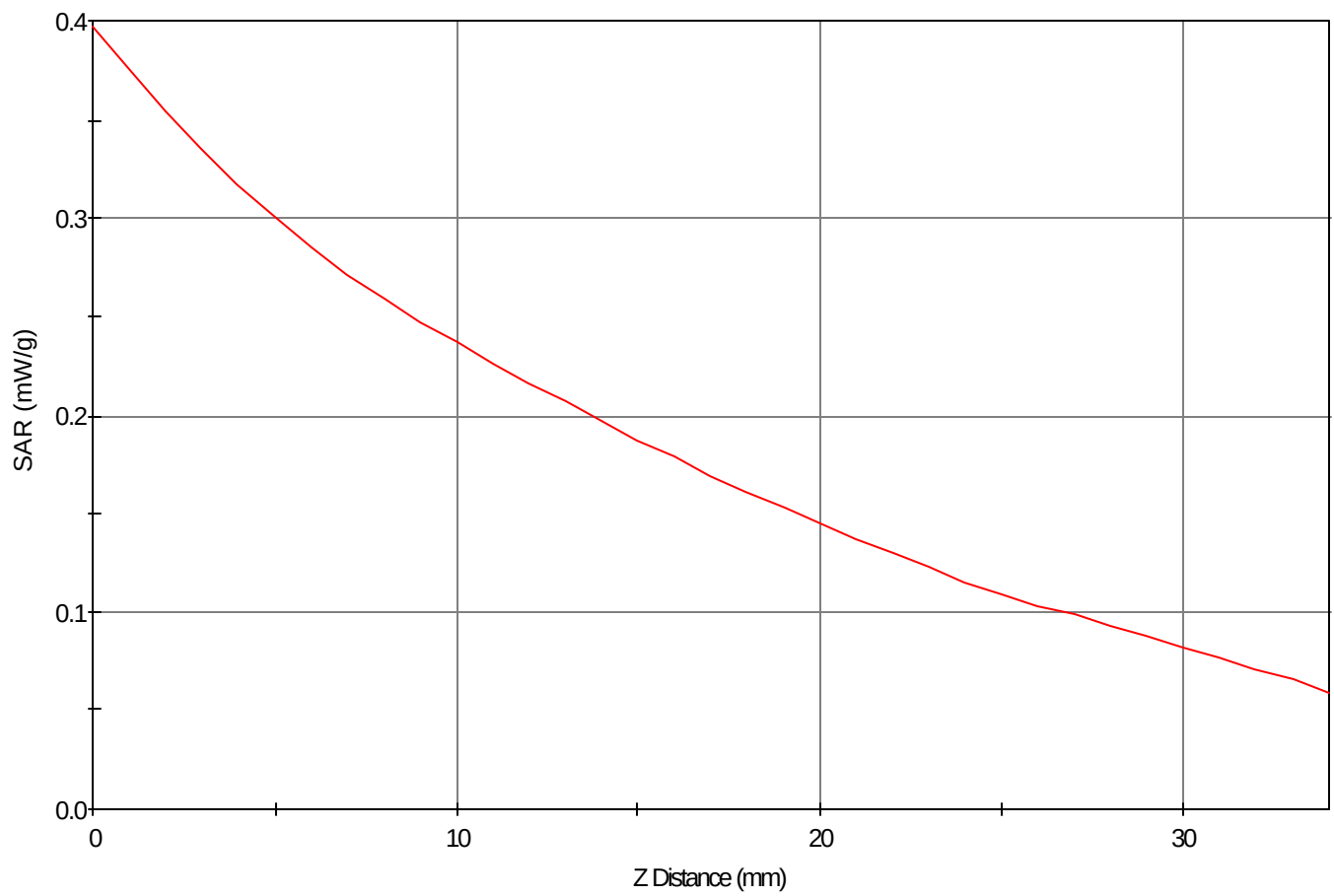
SAR - Z Axis at Hotspot x:58.0 y:14.0
