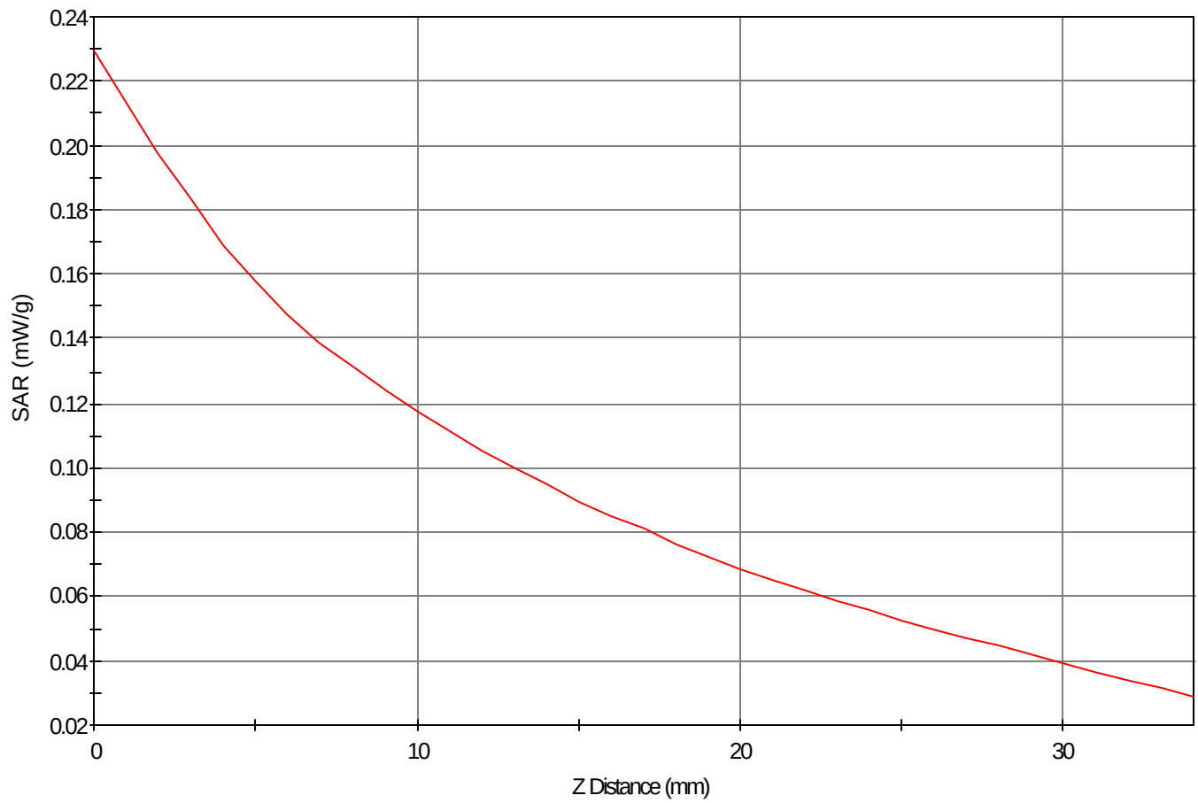
SAR - Z Axis at Hotspot x:28.0 y:7.0
