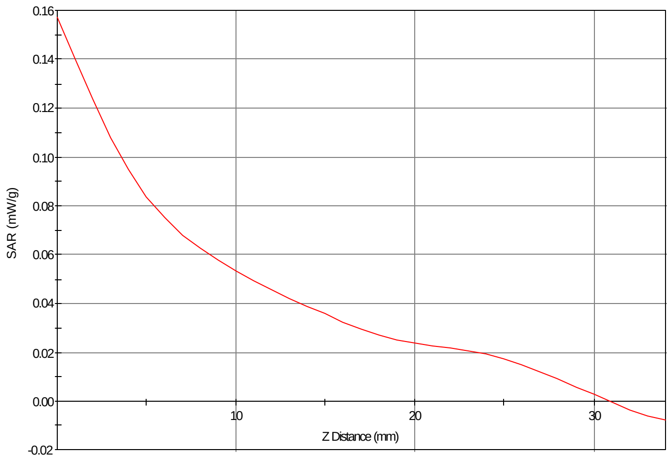
SAR - Z Axis at Hotspot x:6.0 y:6.0
