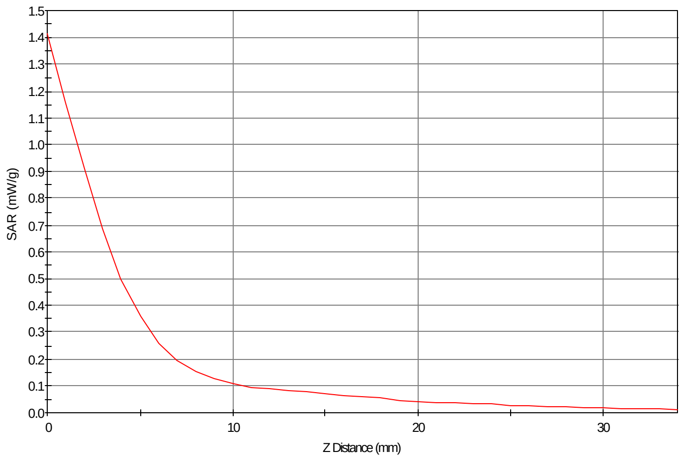
SAR - Z Axis at Hotspot x:-2.0 y:-17.0
