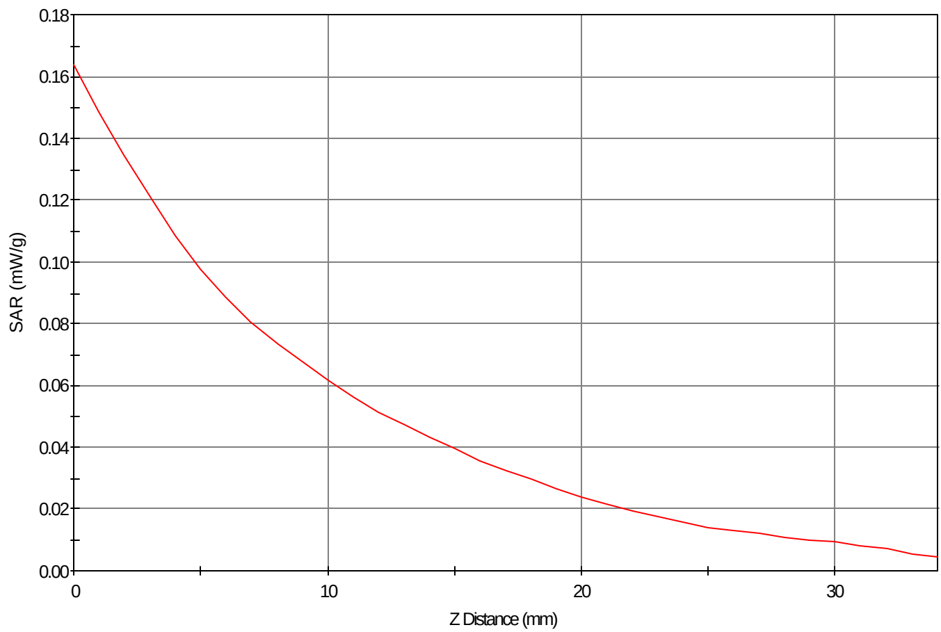
SAR - Z Axis at Hotspot x:60.0 y:20.0
