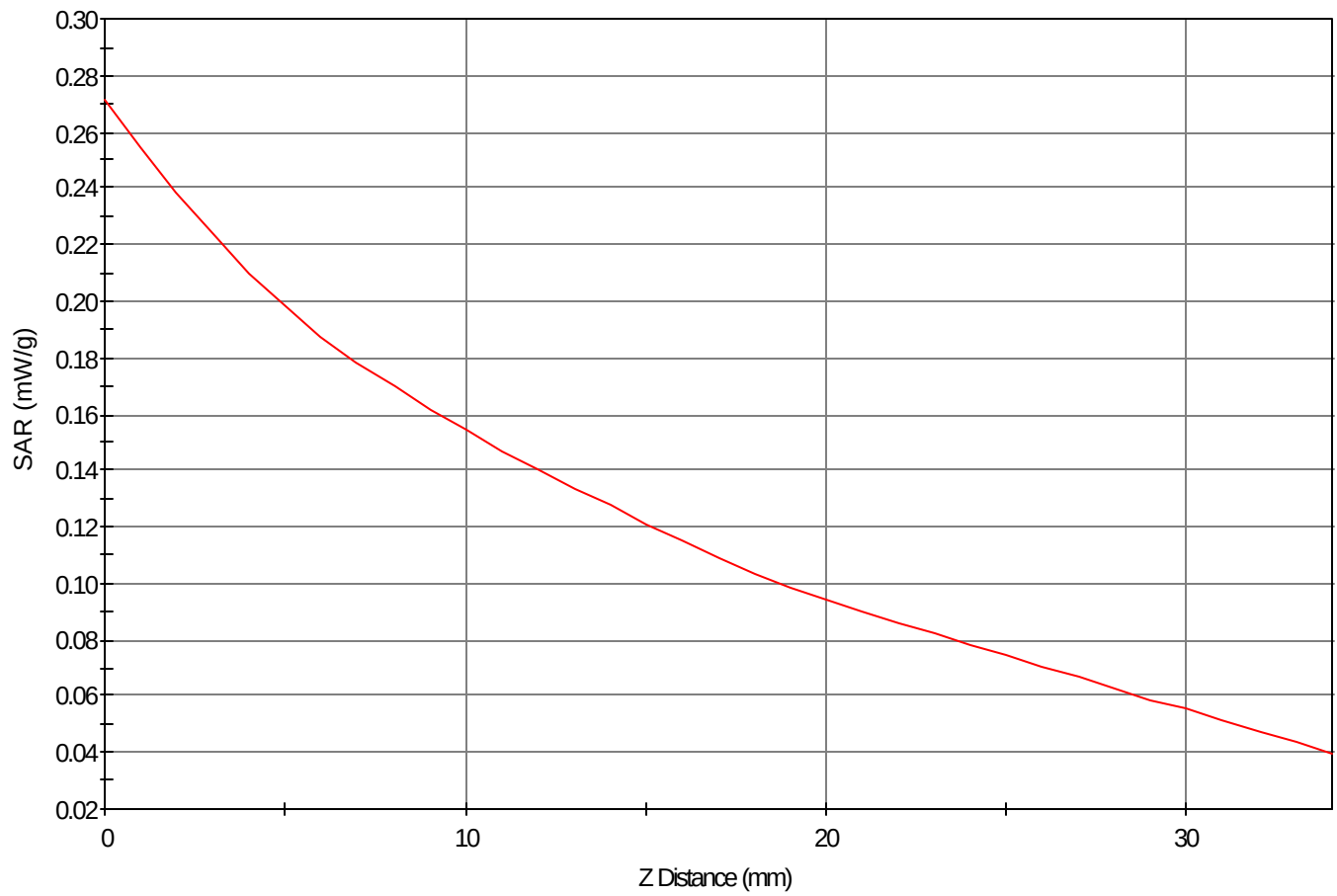
SAR - Z Axis at Hotspot x:35.0 y:11.0
