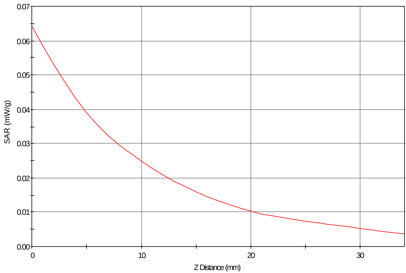
SAR - Z Axis at Hotspot x:17.0 y:-13.0
