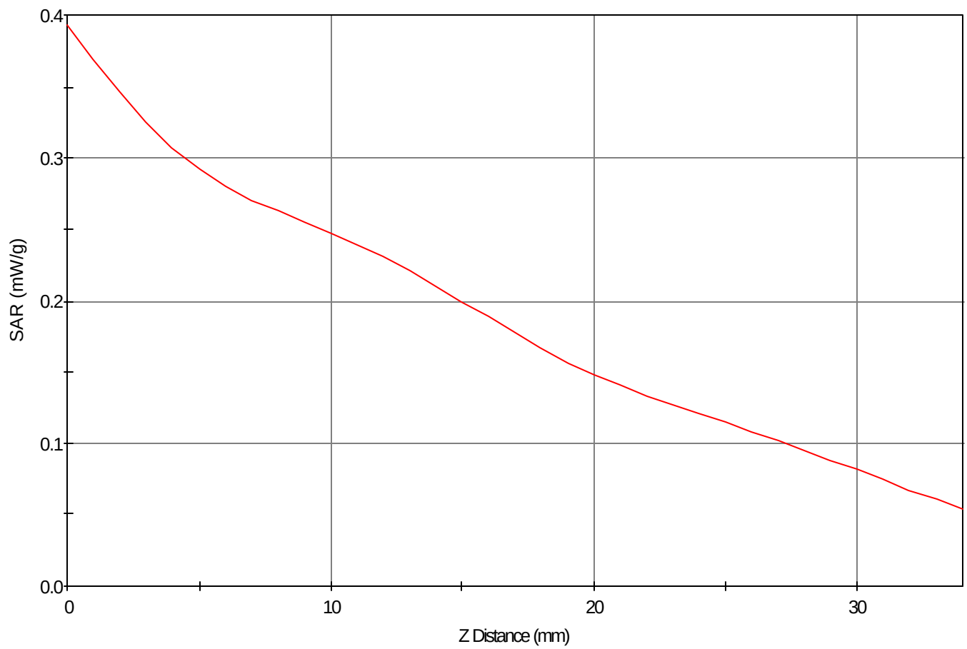
SAR - Z Axis at Hotspot x:52.0 y:8.0
