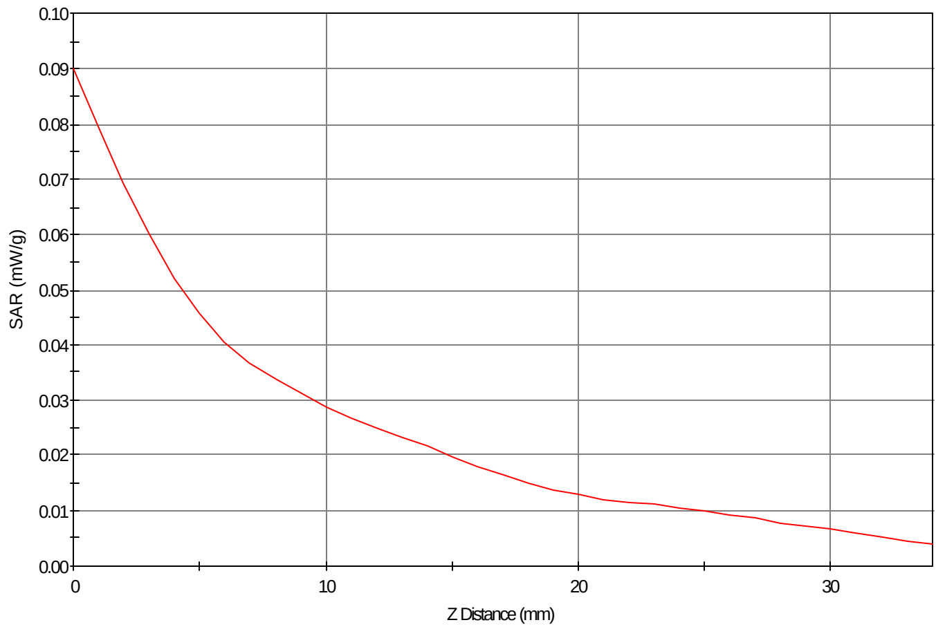
SAR - Z Axis at Hotspot x:80.0 y:25.0
