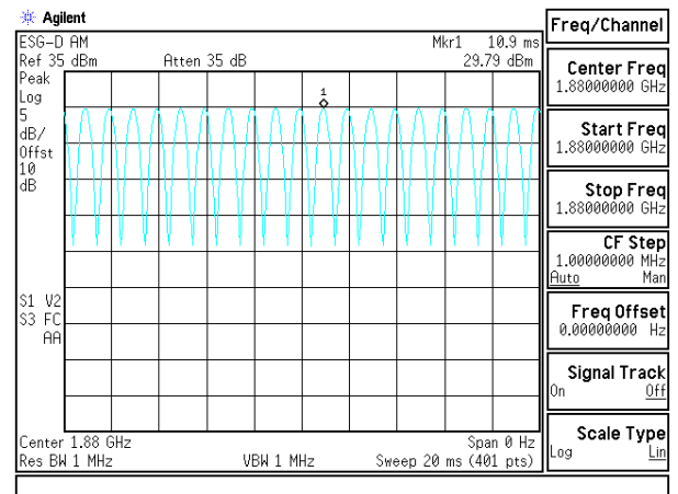
Figure 25 80% AM Signal
