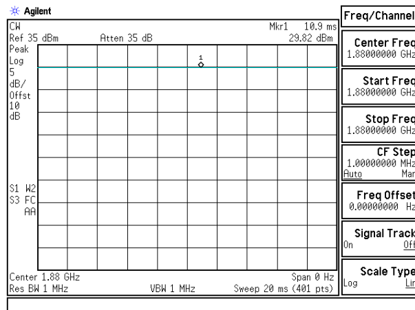
Figure 24 CW Signal
