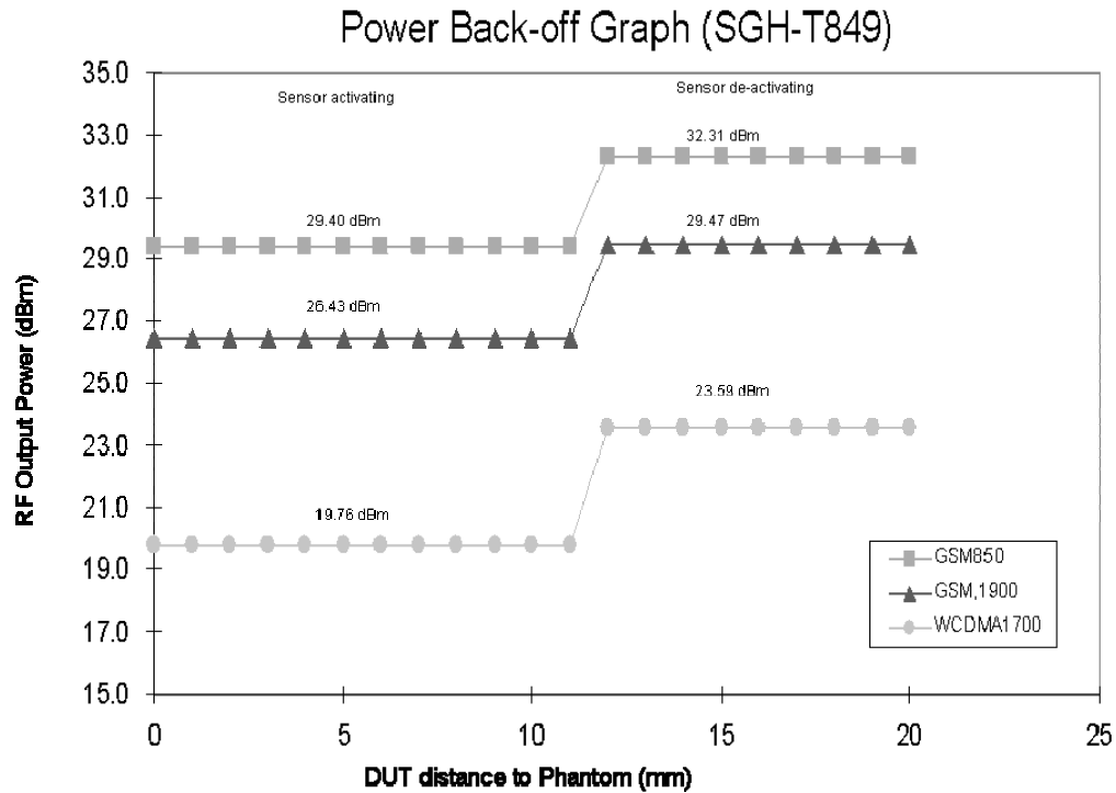
Figure 15-1 Back Off Power Reduction Graph
