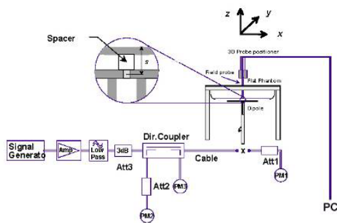
Figure 10-1 System Verification Setup Diagram
