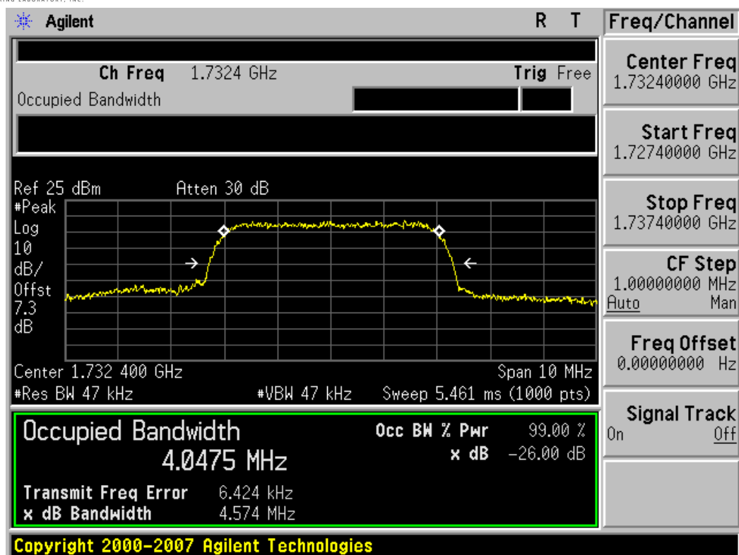
Plot 7-29. Occupied Bandwidth Plot (AWS WCDMA Mode – Ch. 1412)
