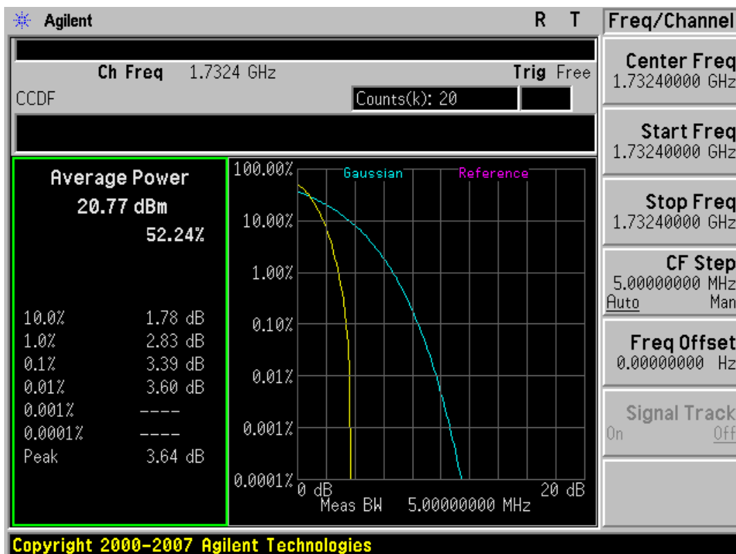
Plot 7-30. Peak-Average Ratio Plot (AWS WCDMA Mode – Ch. 1412)
