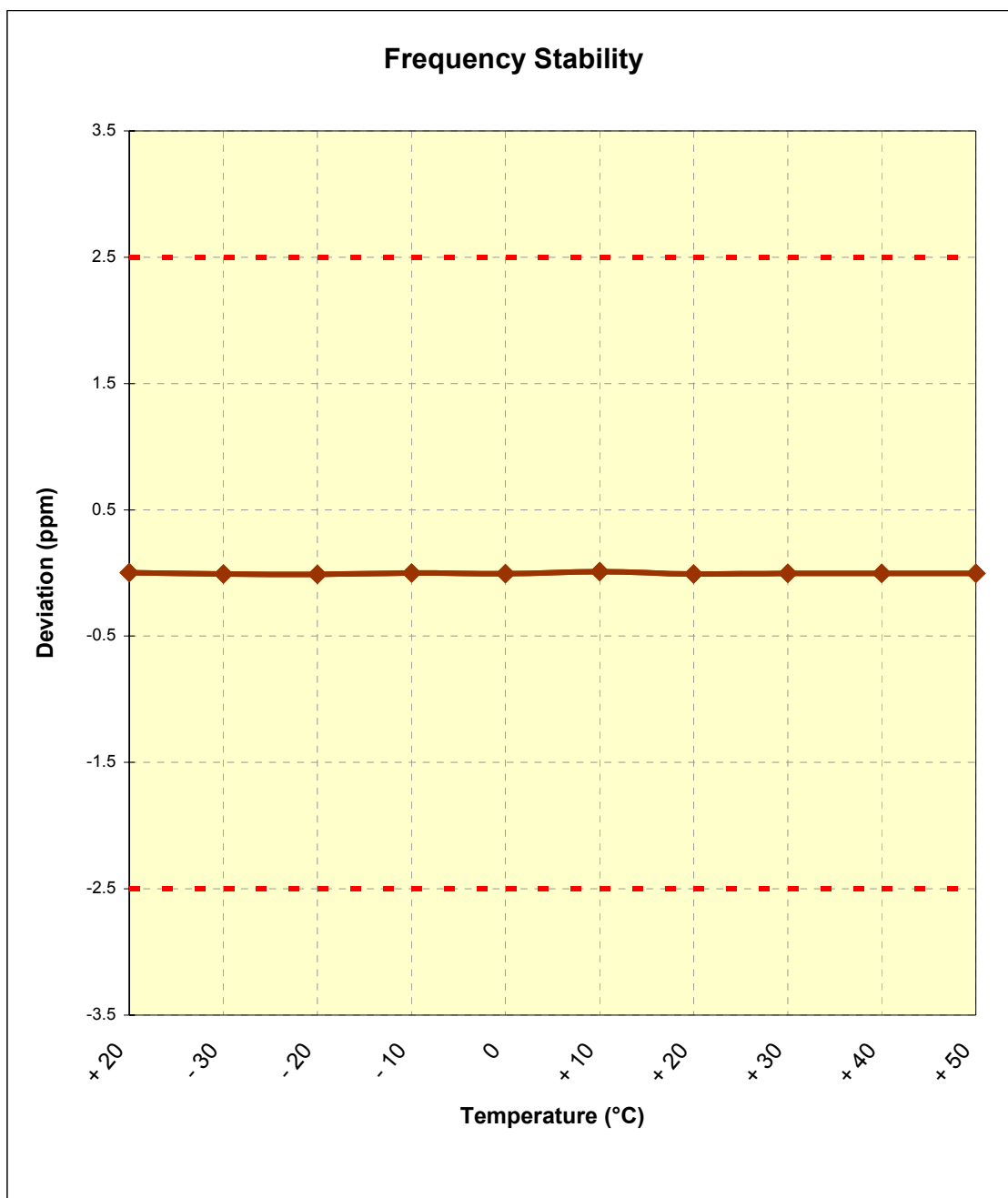
Figure 6-3. Frequency Stability Graph (AWS WCDMA Mode – Ch. 1412)
