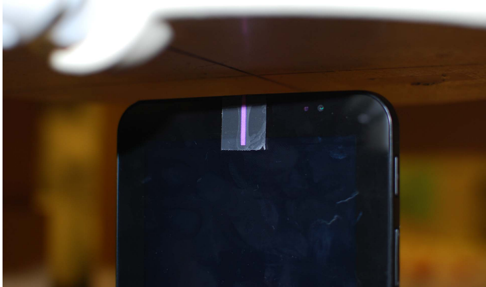
Figure 20-3 SAR Test Setup Photo 2 - Top at 0.5 cm
